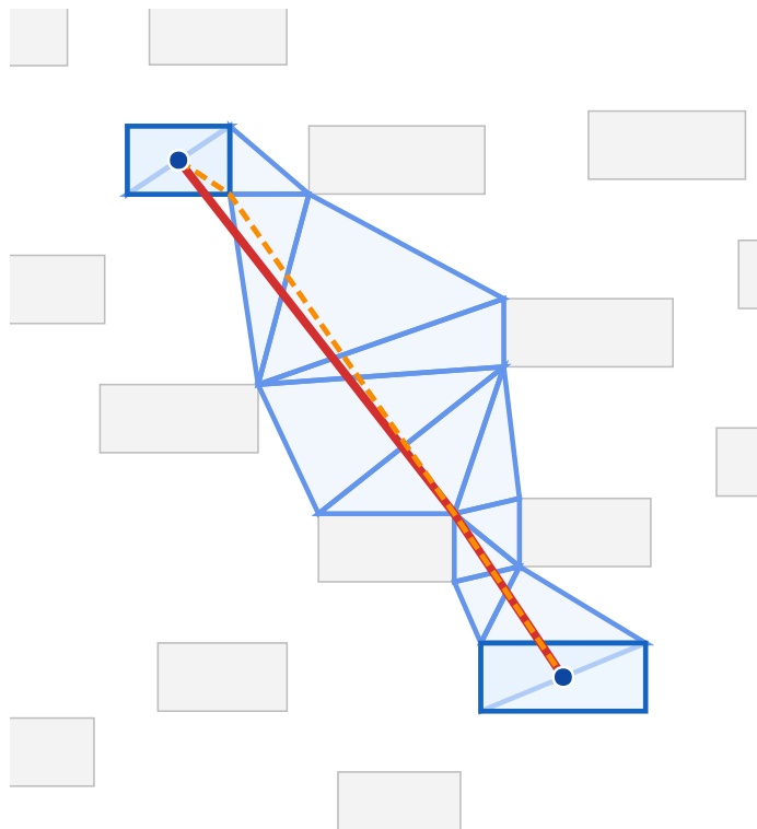
325 Figure 2 Effect of vertex collapse on the OSHA-SMALLJON edge of the Game of Thrones graph. 326 Light blue: the 12-triangle sleeve. Orange dashed: funnel path before collapse (7 waypoints). Red 327 solid: funnel path after collapse (5 waypoints, 21% shorter). Collapsing obstacle vertices to the 328 node center widens the funnel opening at each endpoint and removes the spurious detours around 329 obstacle corners.
