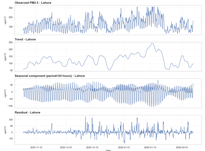
Fig. 6. Seasonal decomposition of cleaned PM_{2.5} series.
