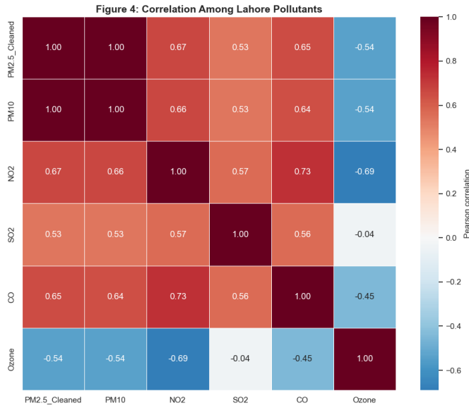
Fig. 4. Correlation matrix among Lahore pollutants.
