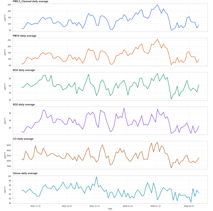
Figure 2: Daily Average Pollutant Concentrations in Lahore
