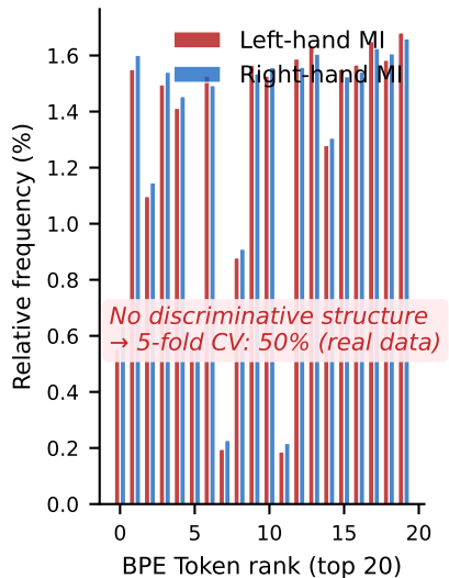
(C) Token histograms per class (top-20 tokens, Left vs Right)
