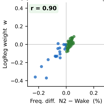
(b) Token enrichment vs weight
