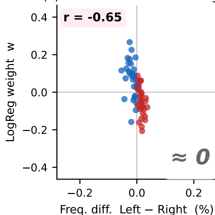
(e) Token enrichment vs weight
