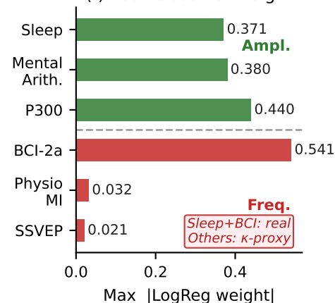
(f) Peak classifier weight
