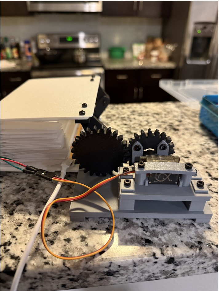
Current build with folded pages
