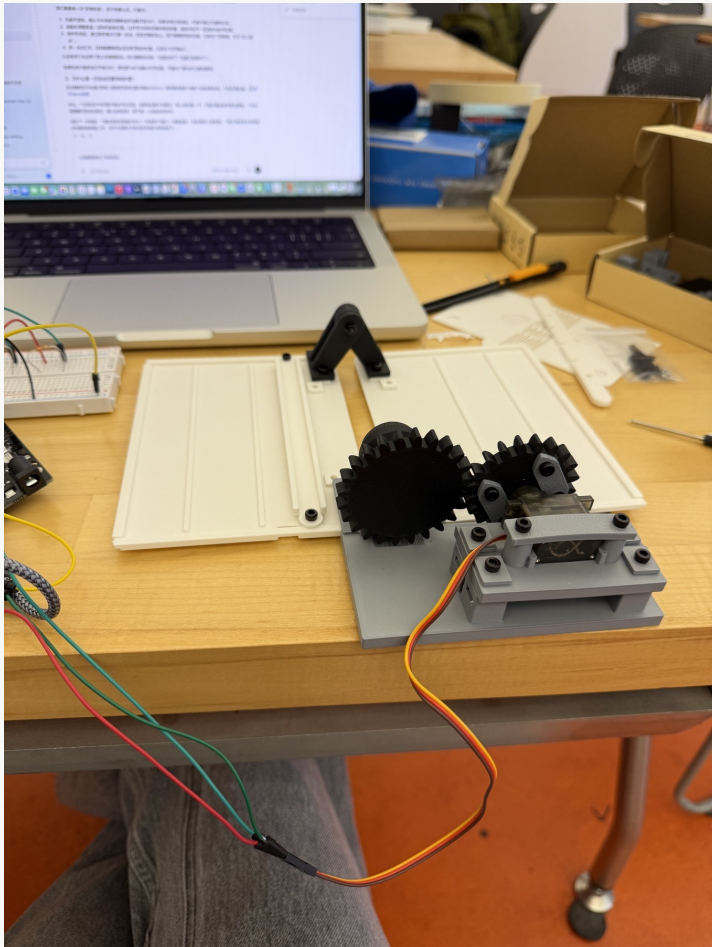
Earlier build, manually positioned open
