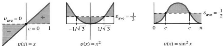
Fig. 5.13 Mean Value Theorem for integrals: area/ (b-a) = average height = v(c) at some c .
