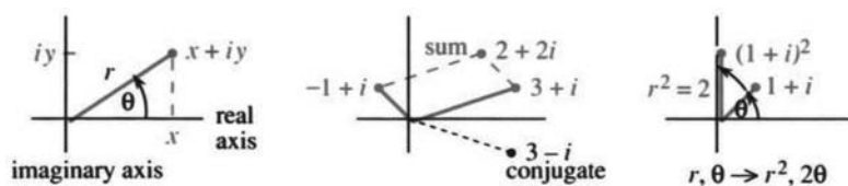
Fig. 9.8 The complex plane shows x , y , r , \theta . Add with x and y , multiply with r and \theta .
