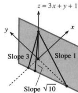
Fig. 11.2 Linear functions give planes.
