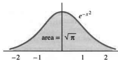
Fig. 14.9 Bell-shaped curve.
