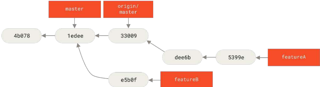
Figure 70. Commit history after featureA work
