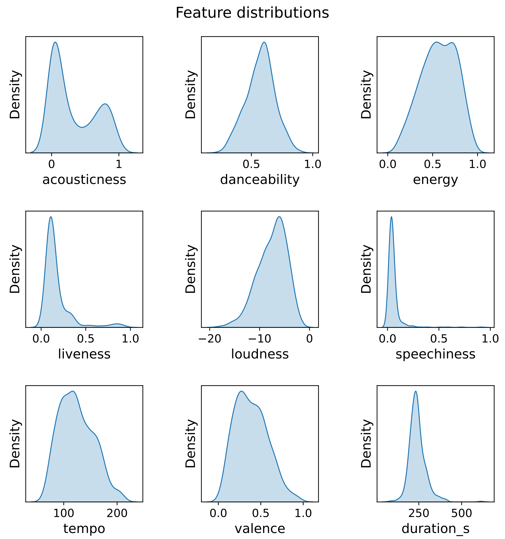
Figure 1: Density estimate plots of musical features.
