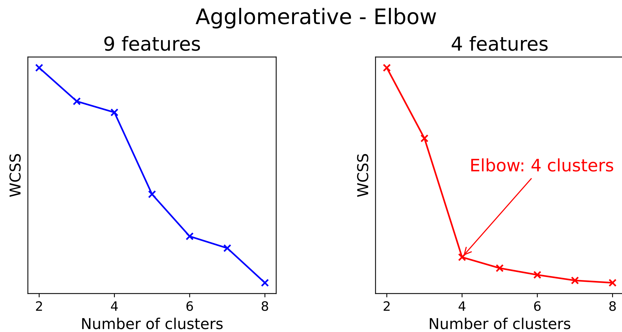
Figure 3: After feature selection, an elbow is present in the WCSS graph.
