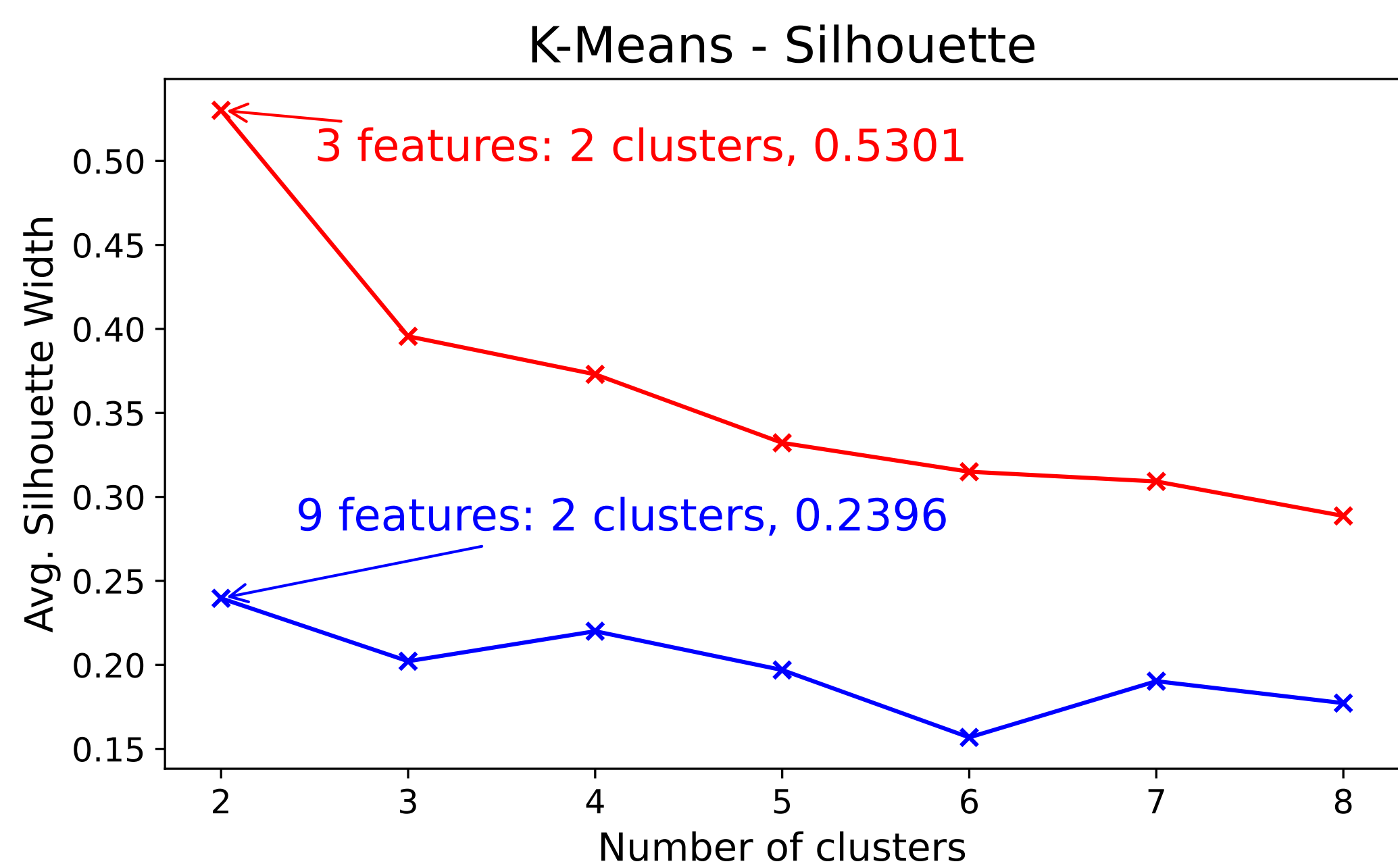
Figure 2: Feature selection reduces noise, creating clearer clusters. This significantly increases average silhouette width while suggesting the same number of clusters.
