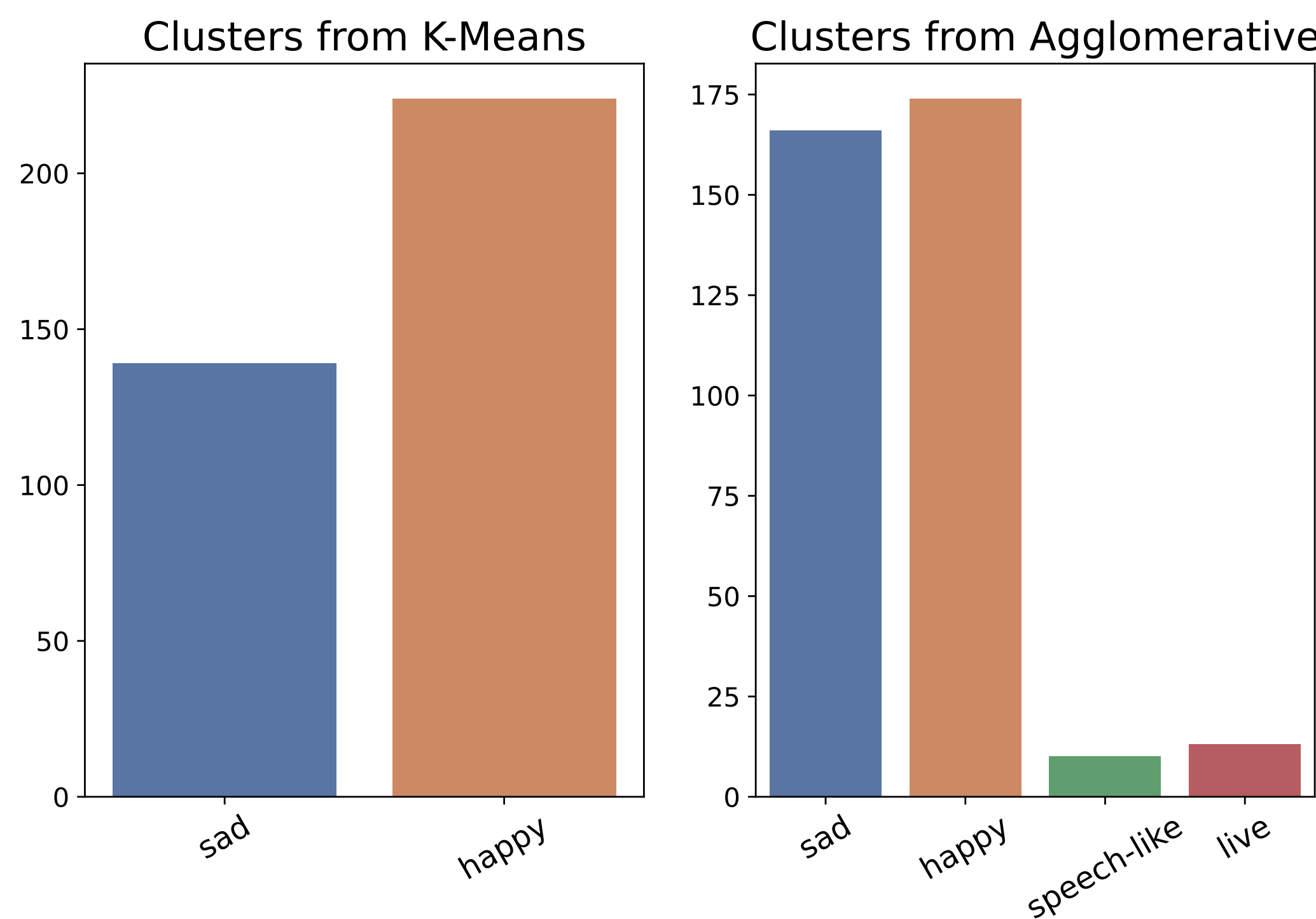
Figure 4: Number of observations in each cluster for both clustering algorithms.
