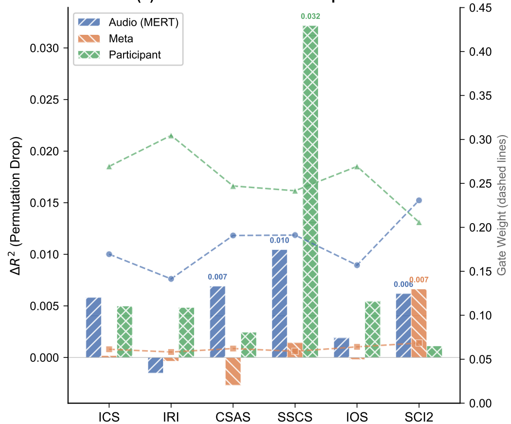
(b) Per-Scale Permutation Importance
