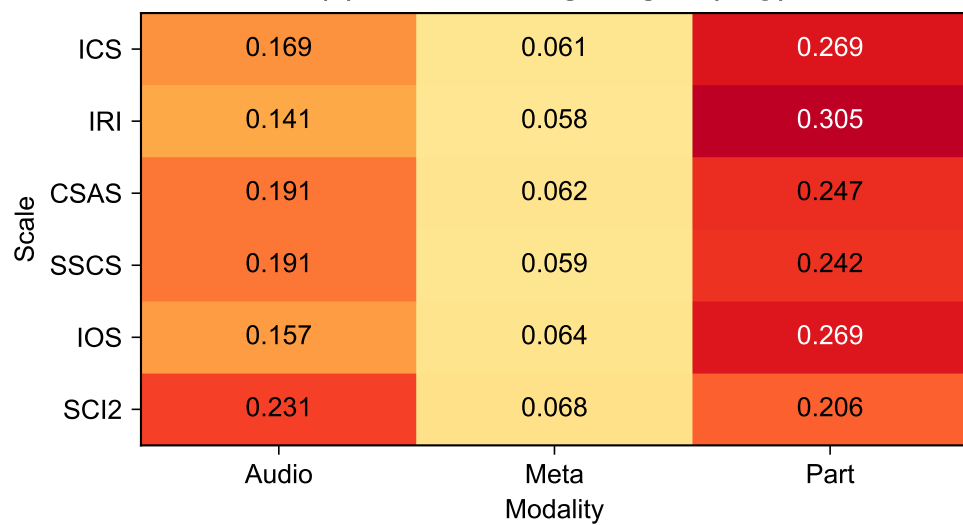
(b) Learned Gating Weights ( \alpha \cdot g )
