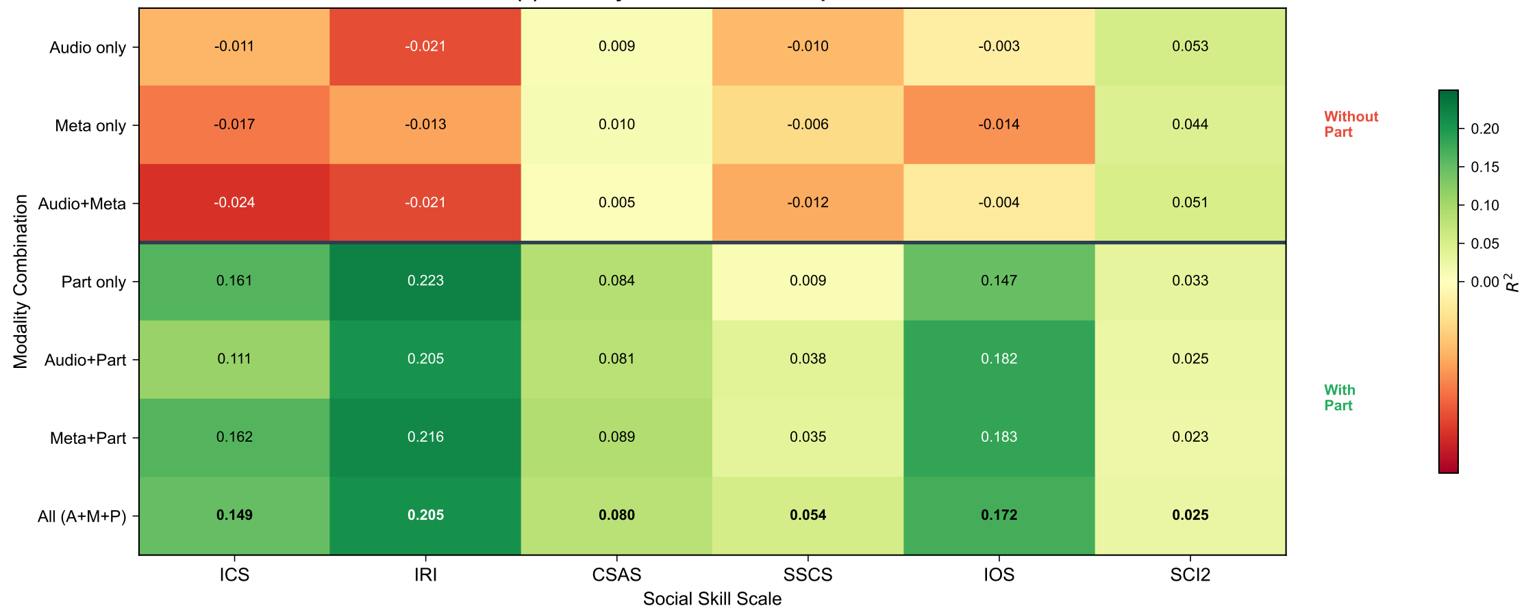
(a) Modality Ablation Matrix: R^2 per Scale
