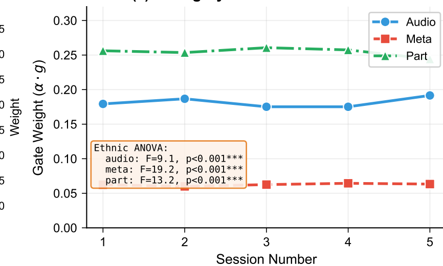
(c) Gating Dynamics Across Sessions
