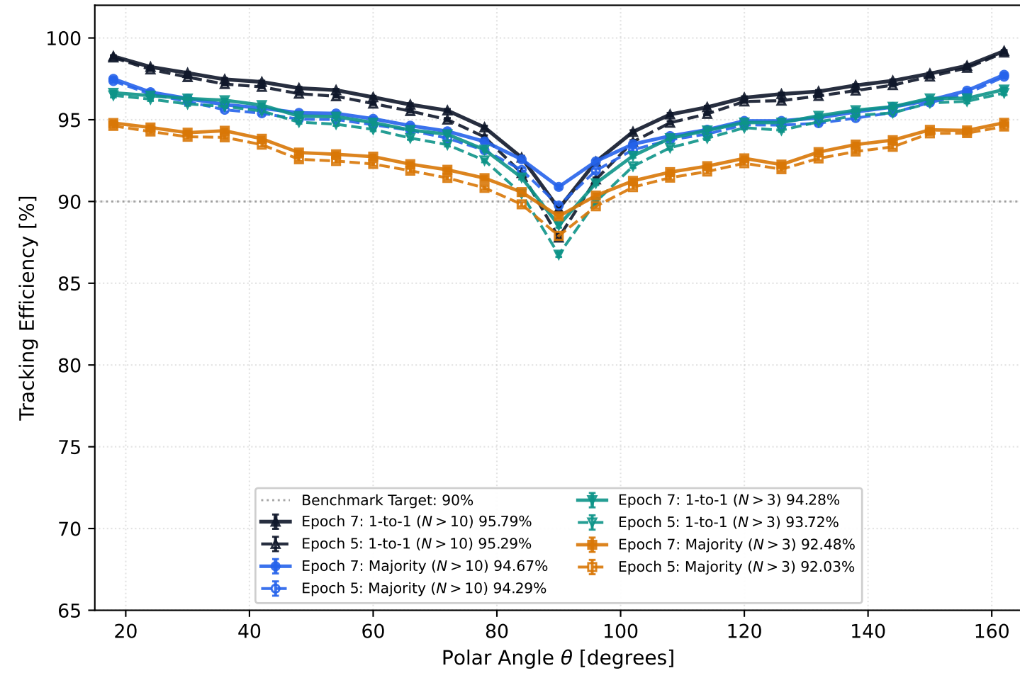
(b) Efficiency vs Polar Angle \theta : Epoch 5 vs Epoch 7 (genStatus \in [0, 1] )
