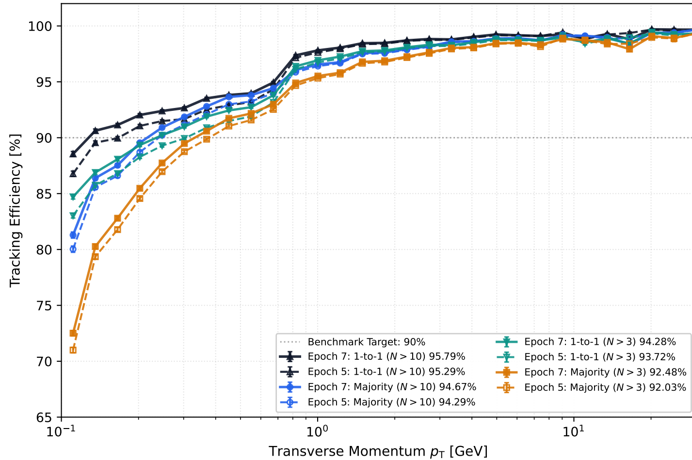
(a) Efficiency vs p_T : Epoch 5 vs Epoch 7 (genStatus \in [0, 1] )
