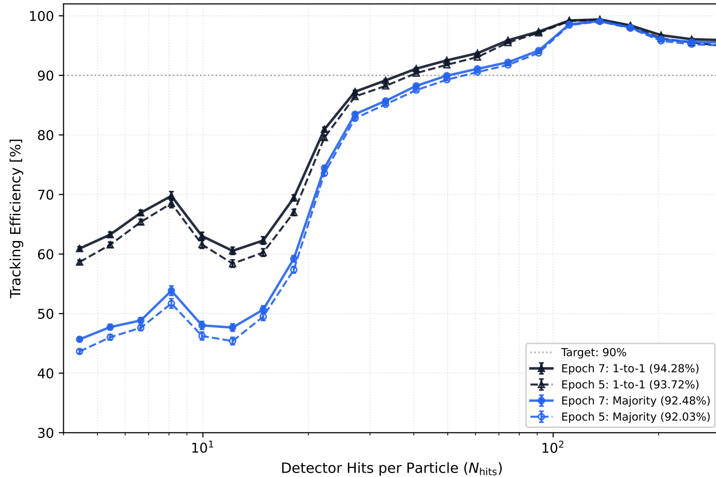
(c) Efficiency vs Hit Multiplicity: Epoch 5 vs Epoch 7 (genStatus \in [0, 1] )
