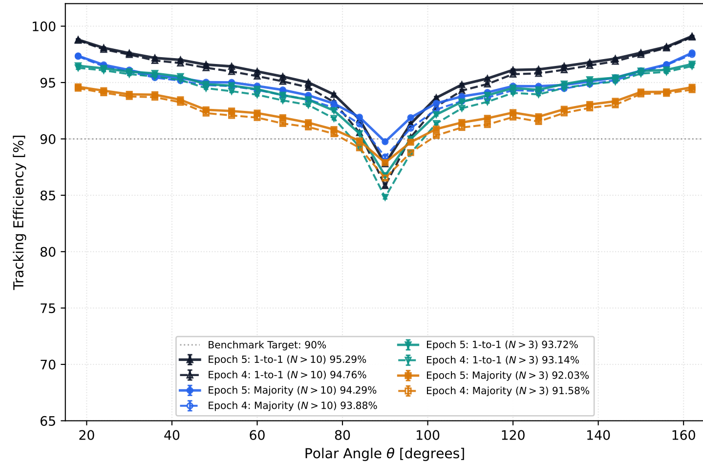
(b) Efficiency vs Polar Angle \theta : Epoch 4 vs Epoch 5 (genStatus \in [0, 1] )
