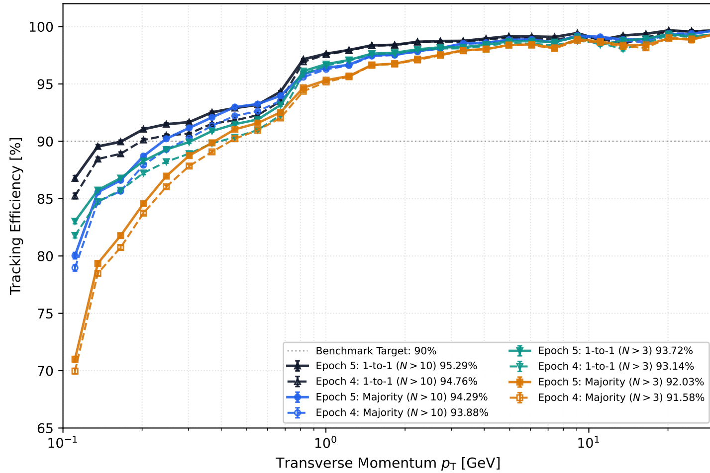
(a) Efficiency vs p_T : Epoch 4 vs Epoch 5 (genStatus \in [0, 1] )
