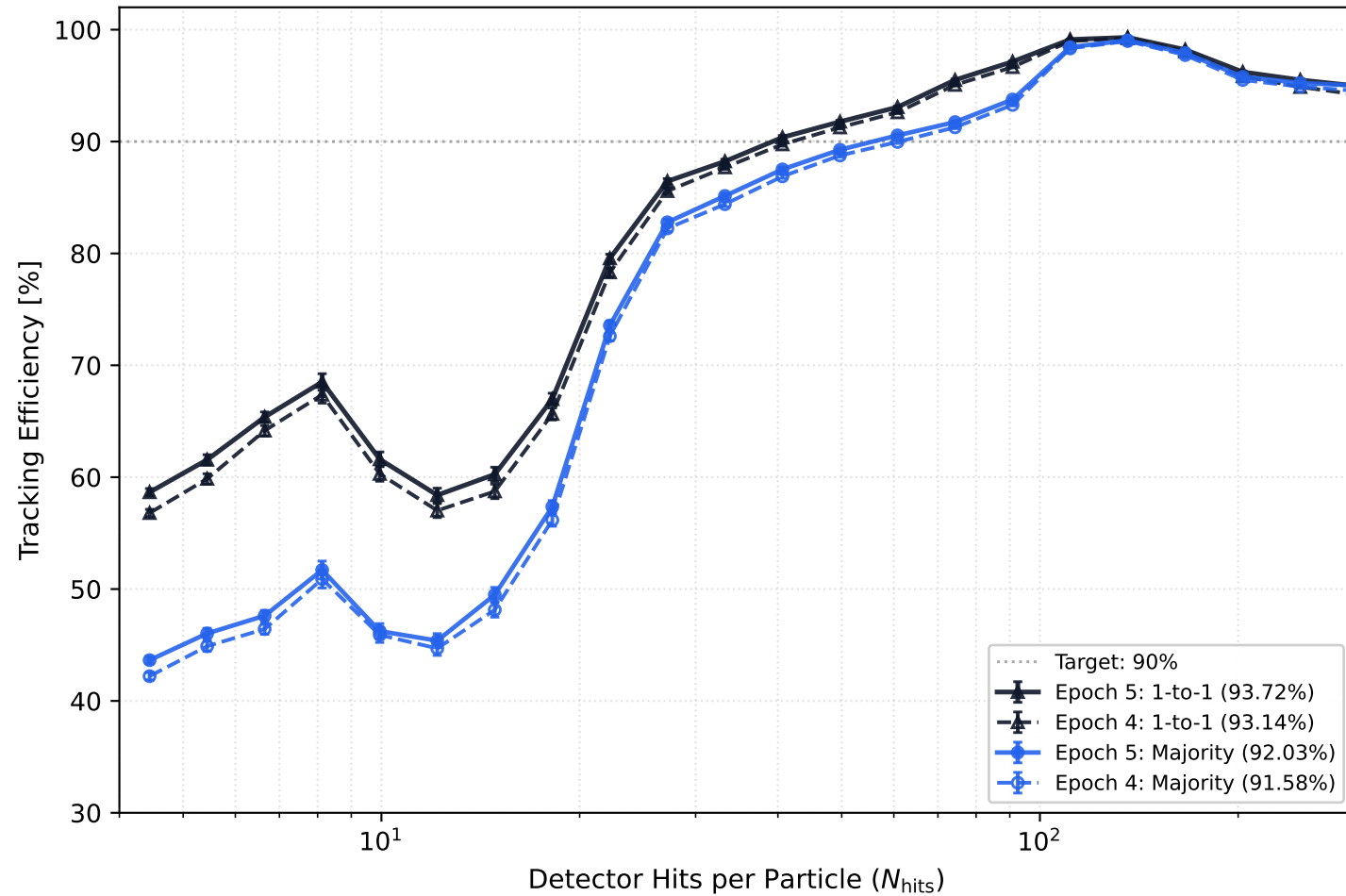
(c) Efficiency vs Hit Multiplicity: Epoch 4 vs Epoch 5 (genStatus \in [0, 1] )
