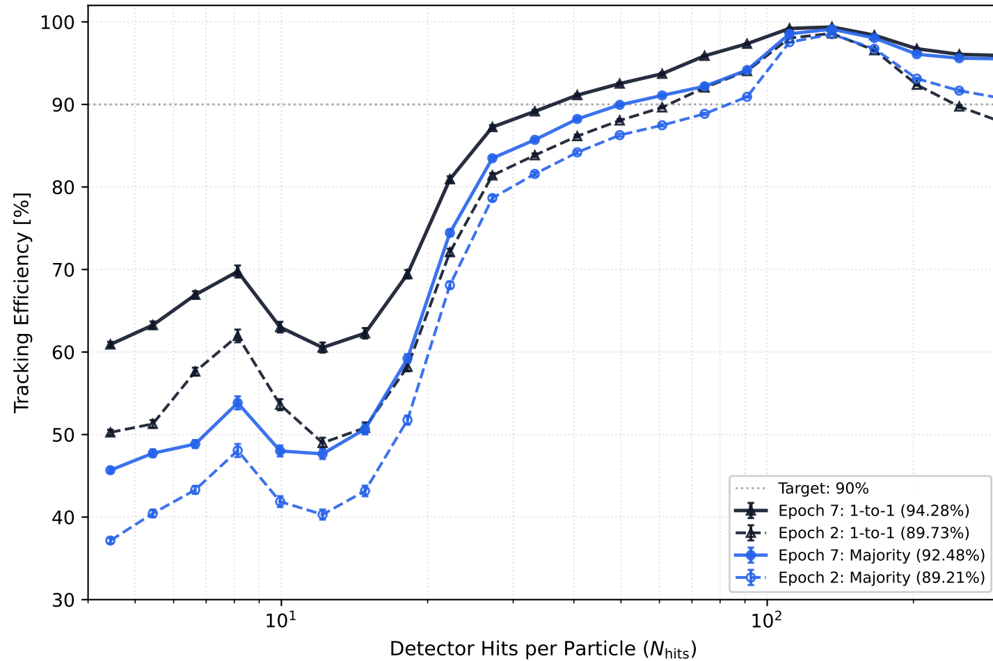
(c) Efficiency vs Hit Multiplicity: Epoch 2 vs Epoch 7 (genStatus \in [0, 1] )
