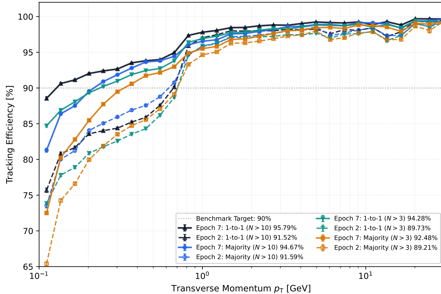
(a) Efficiency vs p_T : Epoch 2 vs Epoch 7 (genStatus \in [0, 1] )
