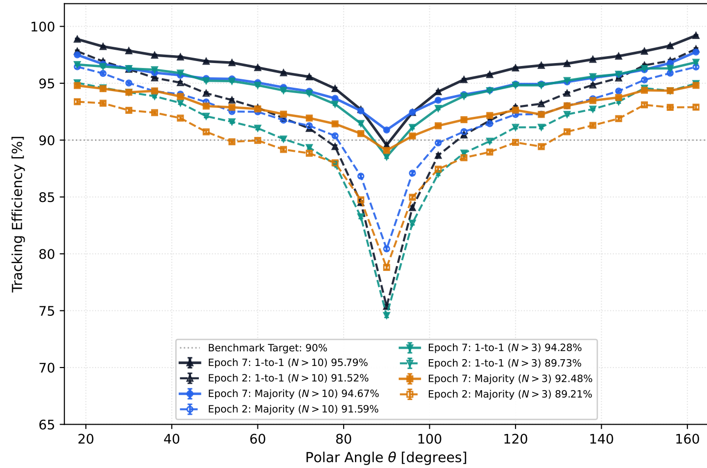
(b) Efficiency vs Polar Angle \theta : Epoch 2 vs Epoch 7 (genStatus \in [0, 1] )
