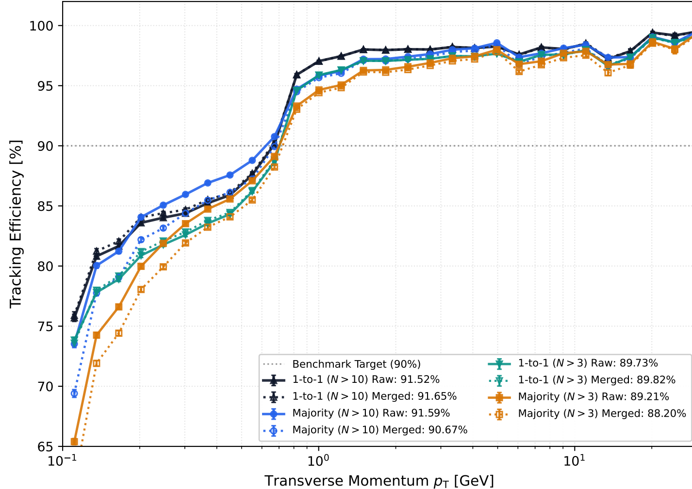
(a) Tracking Efficiency vs p_T ( 15^\circ < \theta < 165^\circ , genStatus \in [0, 1] )
