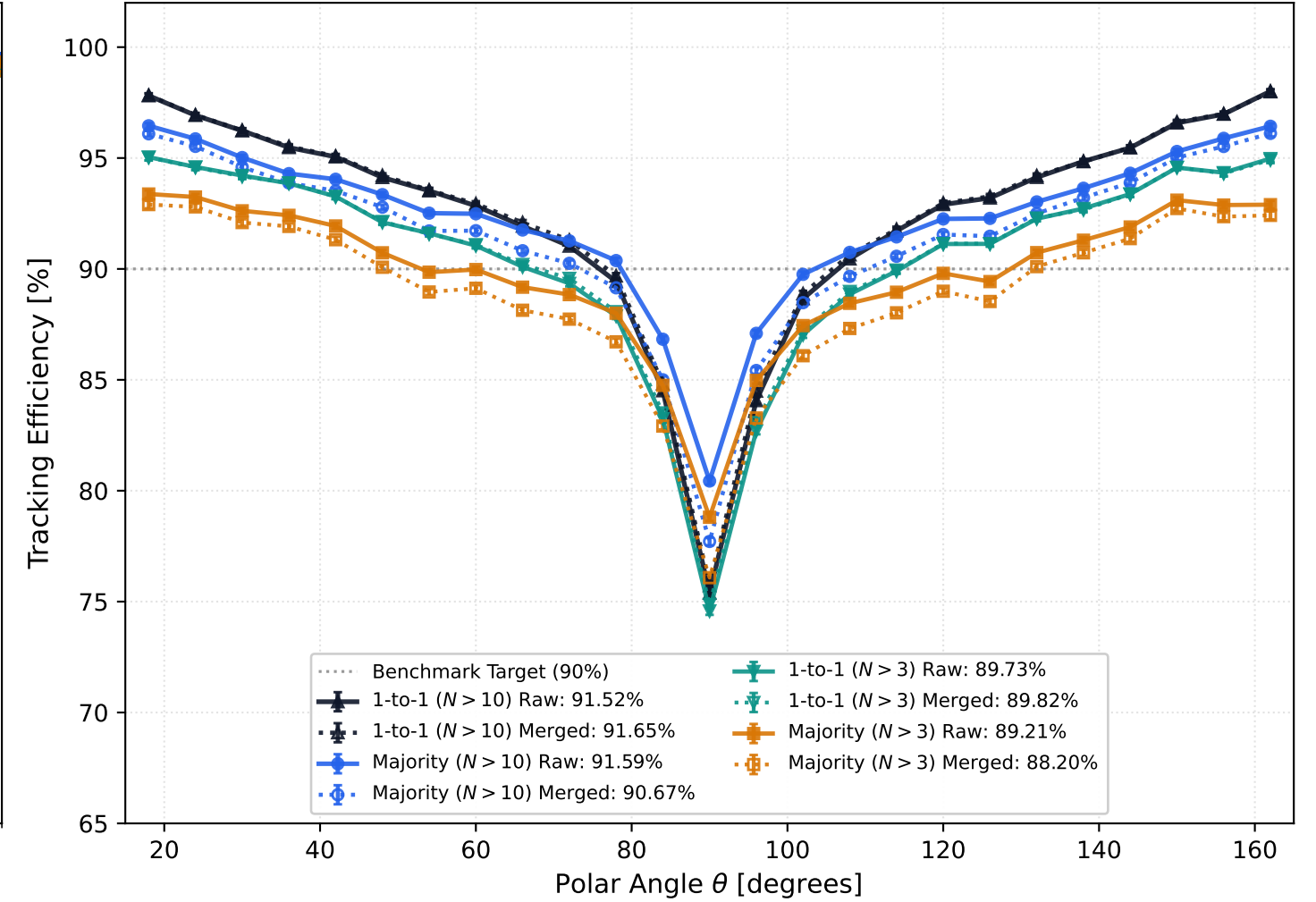
(b) Tracking Efficiency vs Polar Angle Across Acceptance (genStatus \in [0, 1] )
