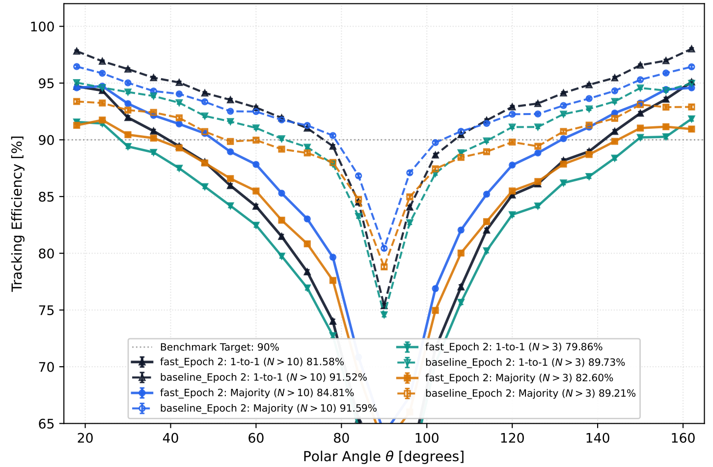
(b) Efficiency vs Polar Angle \theta : baseline_Epoch 2 vs fast_Epoch 2 (genStatus \in [0, 1] )
