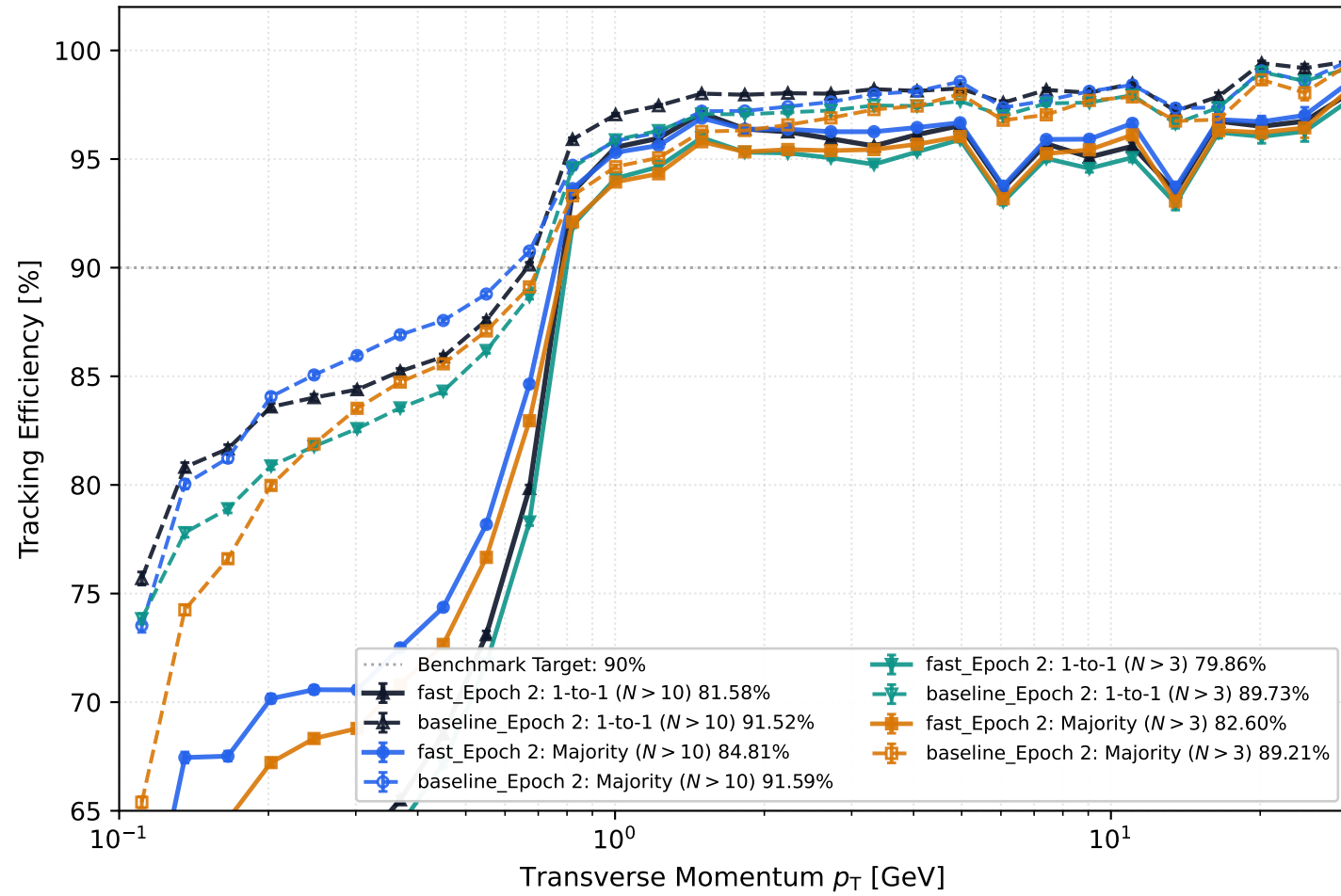
(a) Efficiency vs p_T : baseline_Epoch 2 vs fast_Epoch 2 (genStatus \in [0, 1] )
