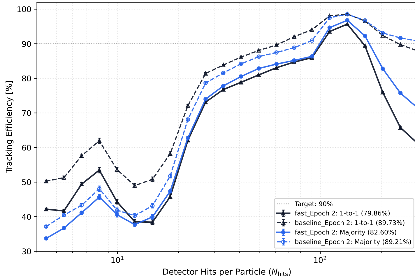
(c) Efficiency vs Hit Multiplicity: baseline_Epoch 2 vs fast_Epoch 2 (genStatus \in [0, 1] )
