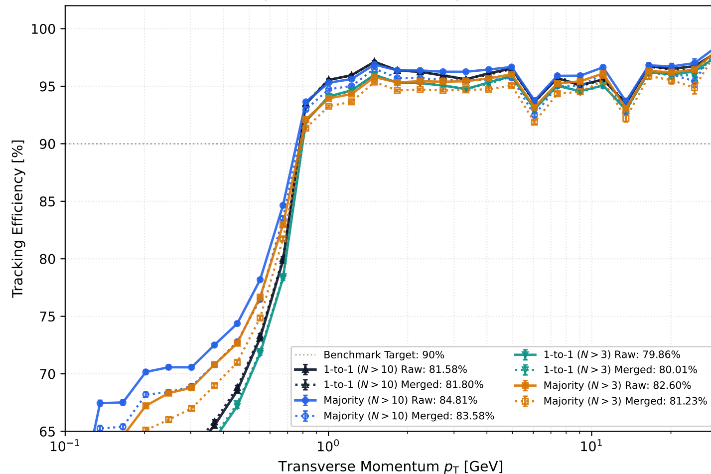
(a) Efficiency vs p_T ( 15^\circ < \theta < 165^\circ , genStatus \in [0, 1] )
