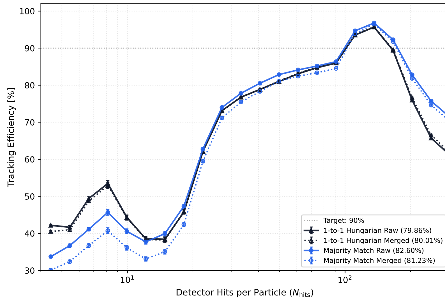
(c) Efficiency vs Hit Multiplicity (Turn-on Curve, genStatus \in [0, 1] )
