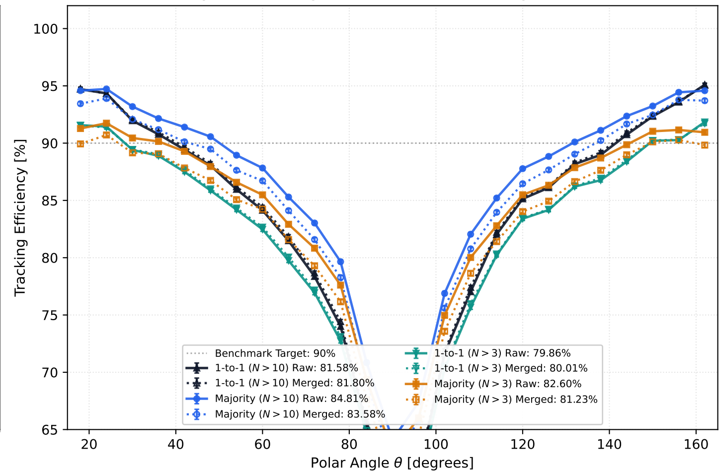
(b) Efficiency vs Polar Angle \theta Across Acceptance (genStatus \in [0, 1] )
