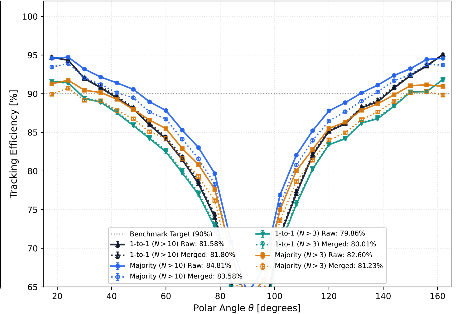
(b) Tracking Efficiency vs Polar Angle Across Acceptance (genStatus \in [0, 1] )
