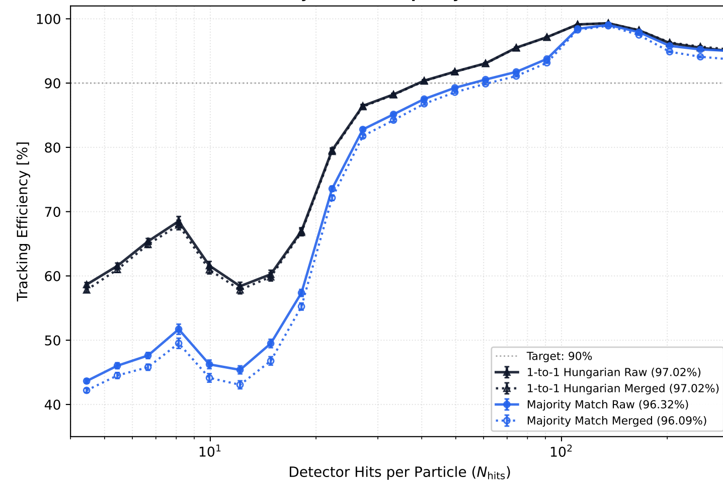
(c) Efficiency vs Hit Multiplicity (Turn-on Curve)
