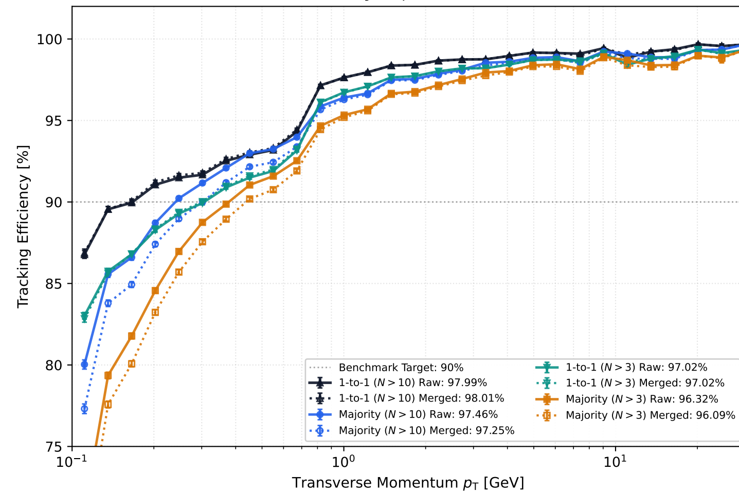
(a) Efficiency vs p_T ( 15^\circ < \theta < 165^\circ )
