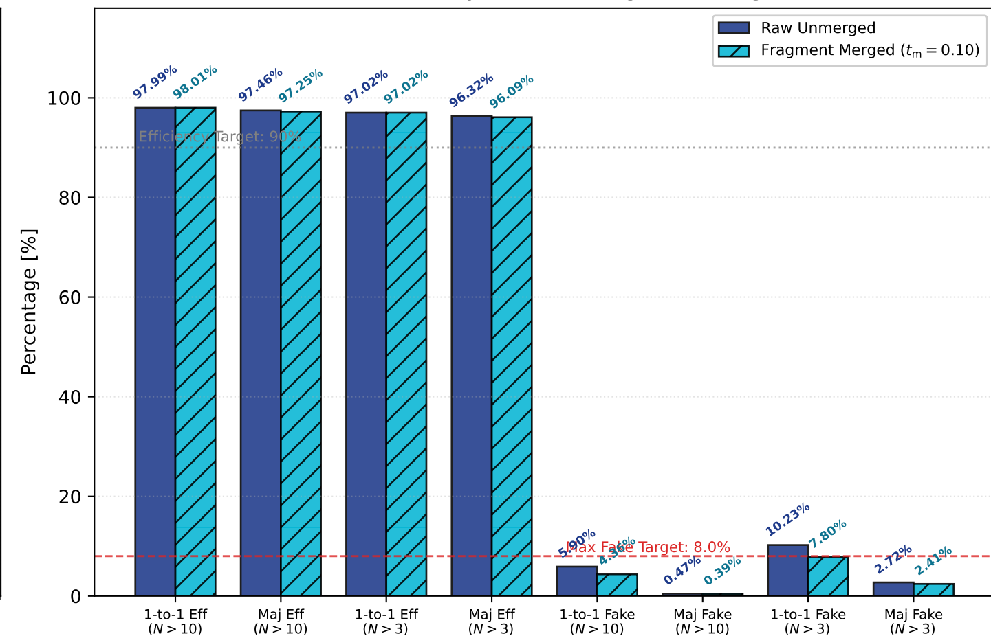
(d) Performance Summary: Raw Unmerged vs Merged ( t_m = 0.10 )
