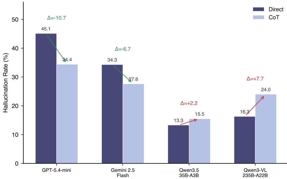
Figure 5.2: Comparison of hallucination rates between Direct and CoT modes. \Delta values indicate the change.
