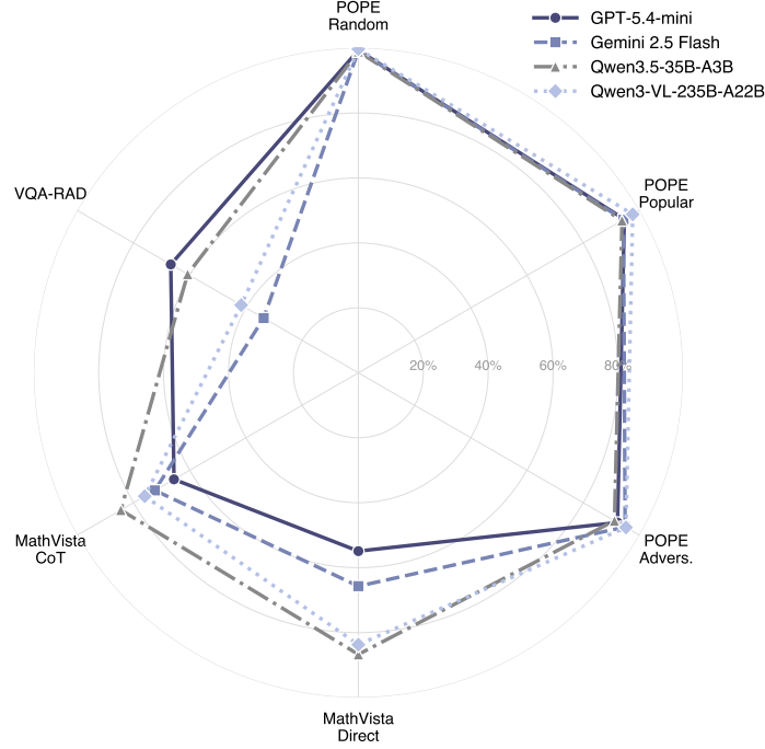
Figure 7.4: Radar chart comparing model performance across six dimensions (accuracy = 1 – HR). Points closer to the outer ring indicate better performance.
