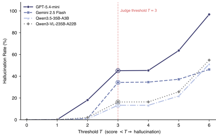
Figure 7.3: Hallucination rate as a function of threshold T (MathVista Direct). The vertical dashed line marks the official threshold T = 3 .
