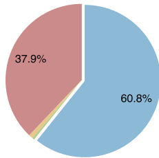
Qwen3.5-35B-A3B
