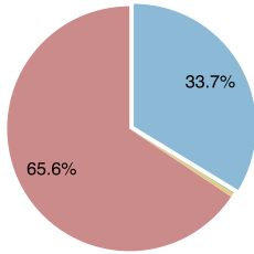
Gemini 2.5 Flash
