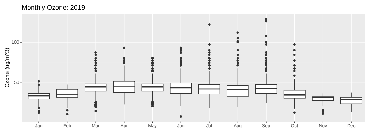
Figure 2: Monthly Ozone (2019)
