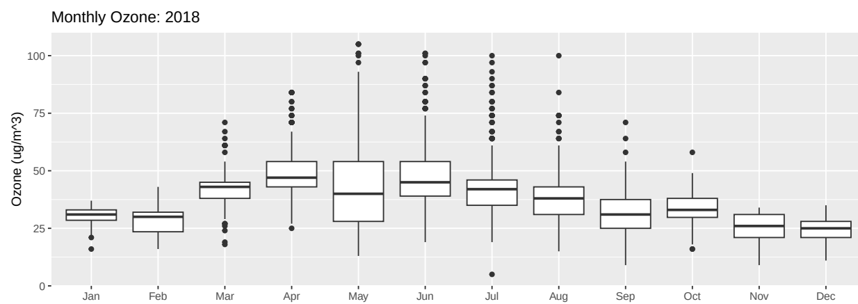
Figure 1: Monthly Ozone (2018)
