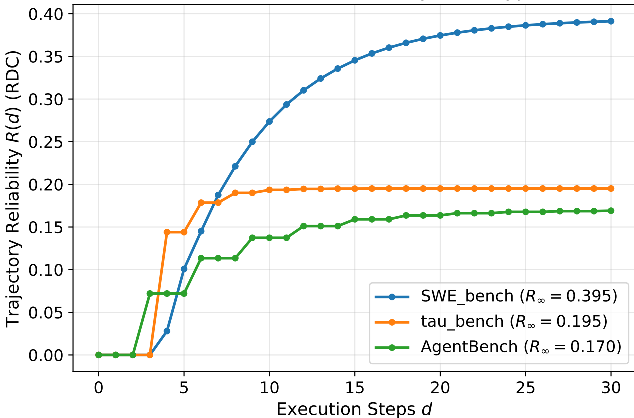
SS7: Cross-Benchmark Generality (Archetype RDC)
