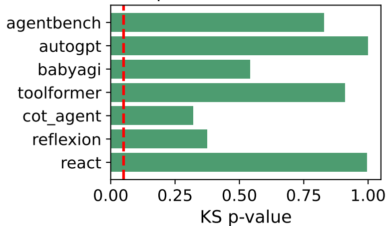
(C) MAST frameworks: per-framework GoF
