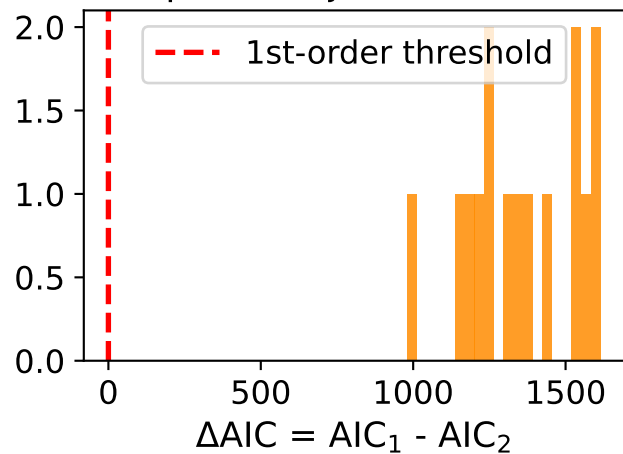
(B) Non-Markov ground truth (mem=0.6) composite reject rate = 1.00
