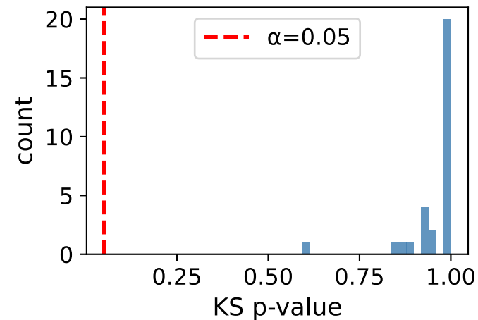
(A) Markov ground truth retain-null rate = 1.00
