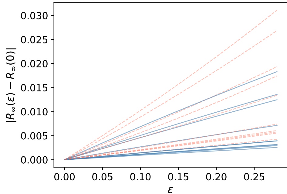
True gap (blue) vs. T2 bound (red dashed)
