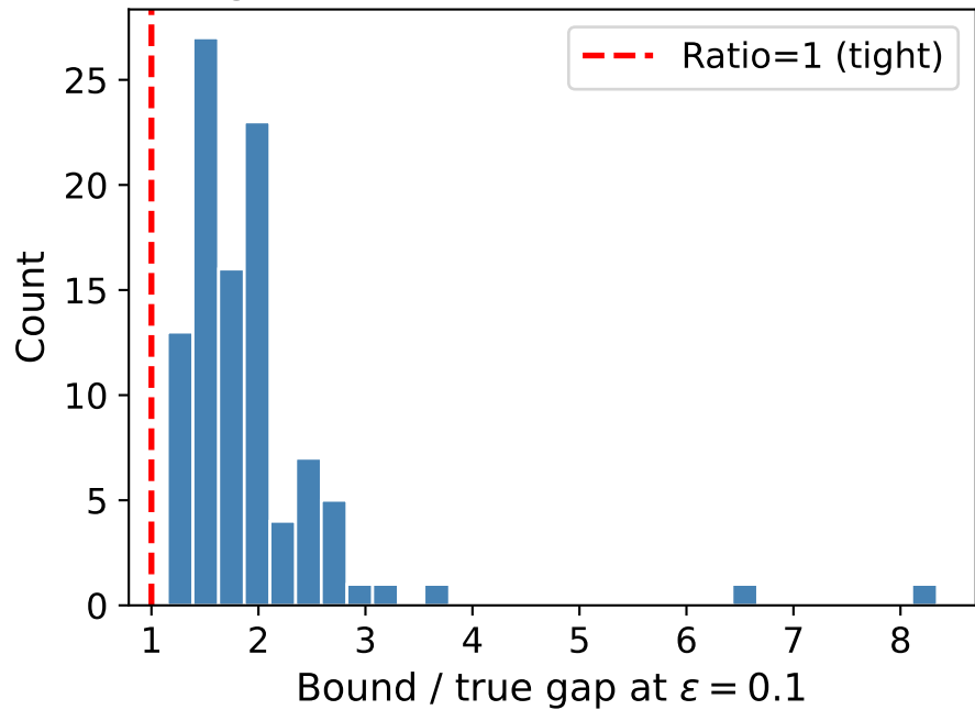
Tightness of T2 bound (100 chains)
