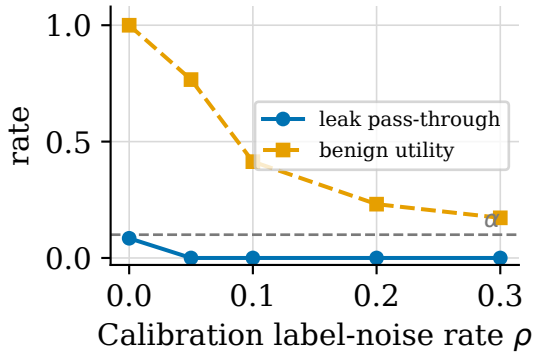
(a) Label noise (PAC)
