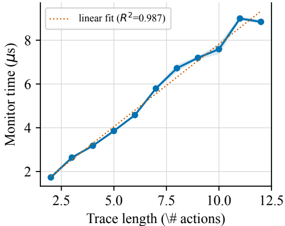
(b) Runtime-monitor scalability
