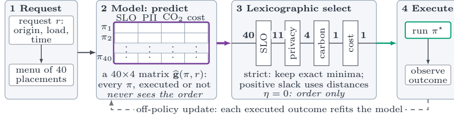
Fig. 1. LEXI’s decision loop: the model predicts every objective for every candidate (purple: the only interface). The strict rule ( \eta = 0 ) reads order only (counts: Table 1).
