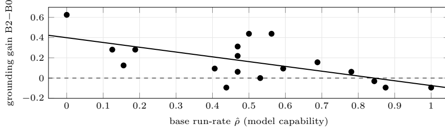
Fig. 4. The crossover: grounding’s repair gain (B2–B0) is large at low capability and turns negative (anchoring) as \hat{\rho} rises. Points are the eighteen models ( n=32 each); the line is the fitted interaction (slope -0.47 , R^2=0.40 ), crossing zero at \hat{\rho} \approx 0.84 .
