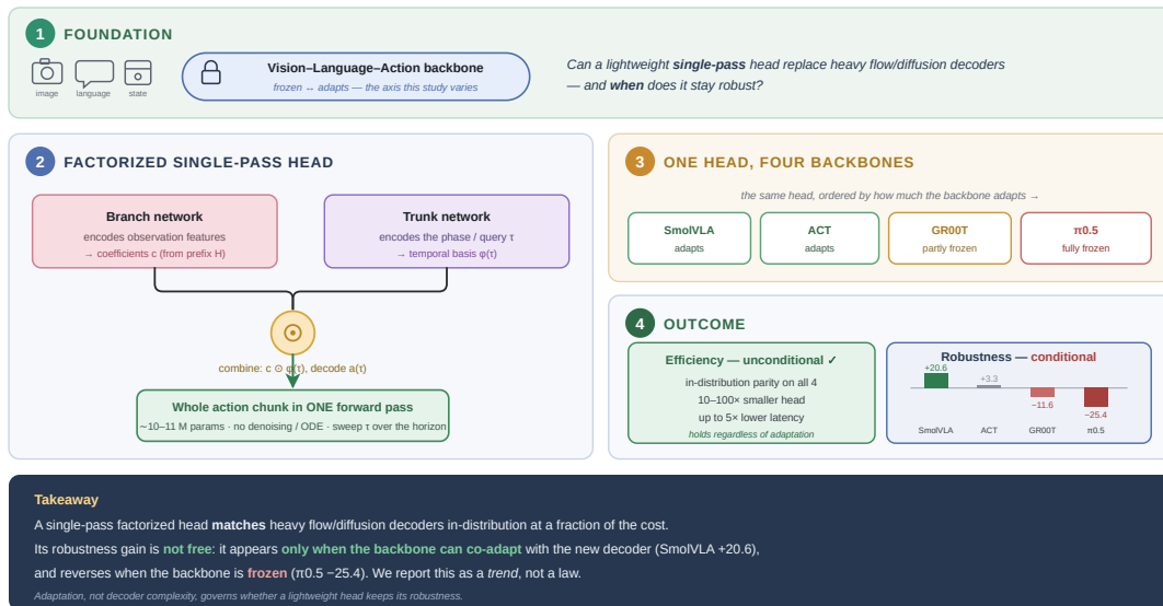
Figure 1. Graphical abstract. We replace a VLA model’s heavy iterative flow/diffusion action head with a single-pass factorized (branch–trunk) head at \sim 10\text{--}11 M parameters. In-distribution accuracy and efficiency improve unconditionally; the robustness effect is conditional and tracks how much the backbone is free to adapt (SmolVLA +20.6 \rightarrow frozen \pi 0.5 −25.4).
