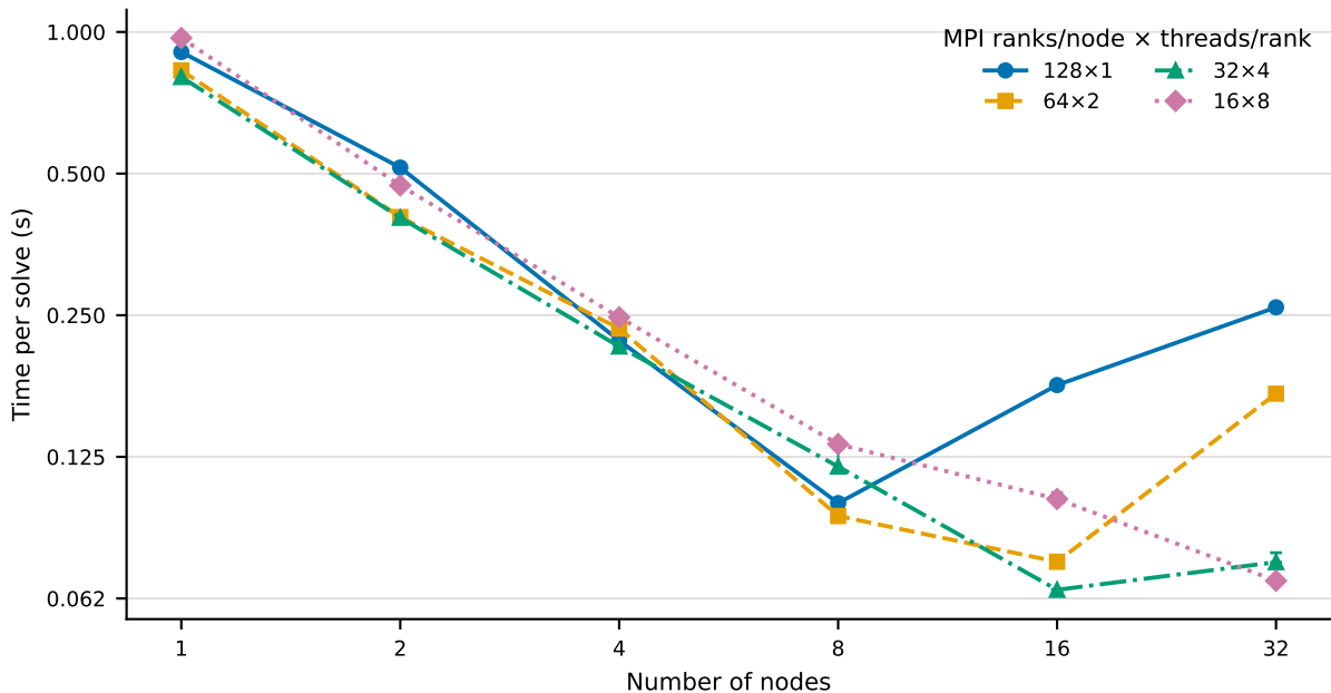
3D PETSc fixed-20m strong scaling: runtime Median across three formal runs
