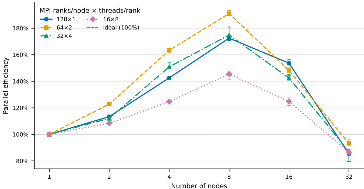
2D PETSc fixed-20m strong scaling: efficiency Median across three formal runs
