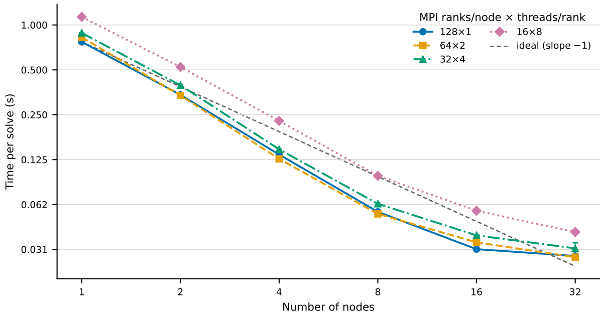
2D PETSc fixed-20m strong scaling: runtime Median across three formal runs
