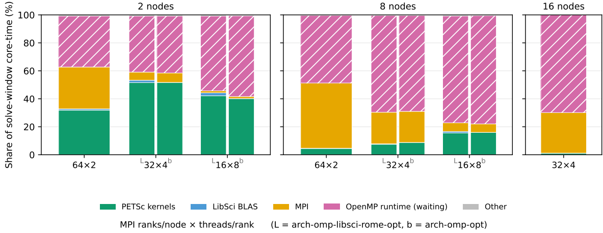
Figure 5.1: Where the cores are during the solve, from the MAP call trees. Within each panel the OpenMP waiting share grows and the MPI share shrinks as threads replace ranks, and both effects strengthen with node count. Paired bars are the two PETSc builds at the same configuration.
