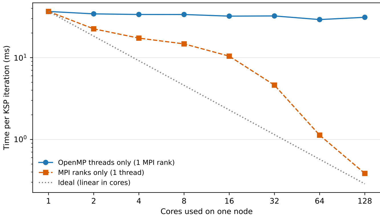
Single-node default-solver sweep: threads do not replace ranks 1000×1000 grid, best of the available repeats
