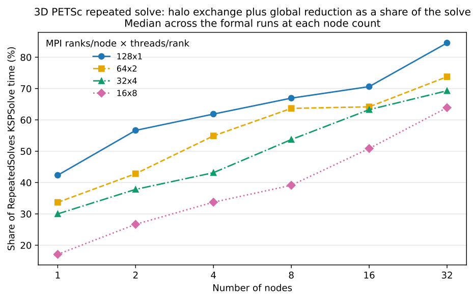
Figure 5.3: 3D share of RepeatedSolves KSPSolve time spent inside halo exchange and global reduction events. Note the vertical scale: flat MPI reaches 84.6% at the largest point.
