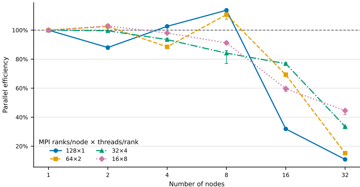
3D PETSc fixed-20m strong scaling: efficiency Median across three formal runs
