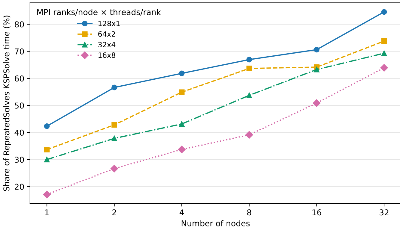
3D PETSc repeated solve: halo exchange plus global reduction as a share of the solve Median across the formal runs at each node count
