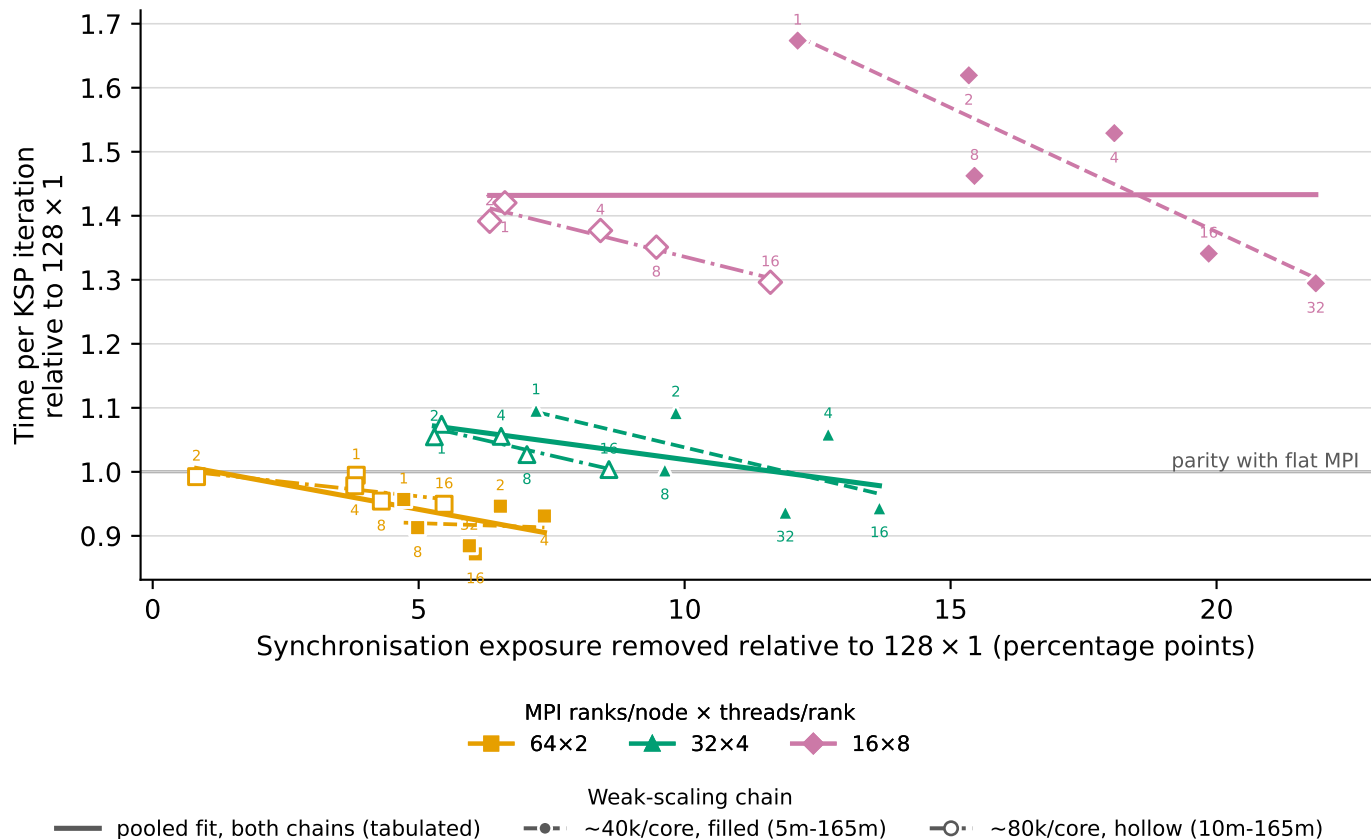
2D: exposure removed against the speed it buys Point labels are node counts; fits are descriptive and clipped to their data
