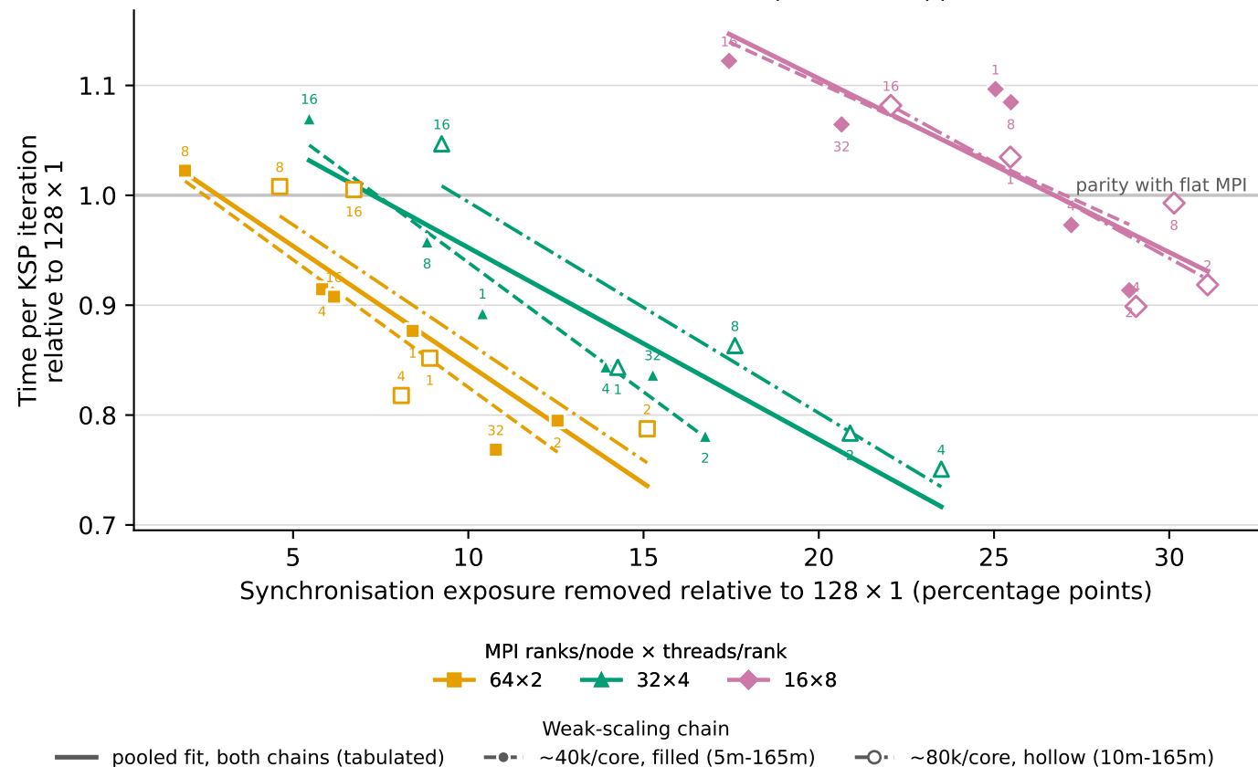
3D: exposure removed against the speed it buys Point labels are node counts; fits are descriptive and clipped to their data
