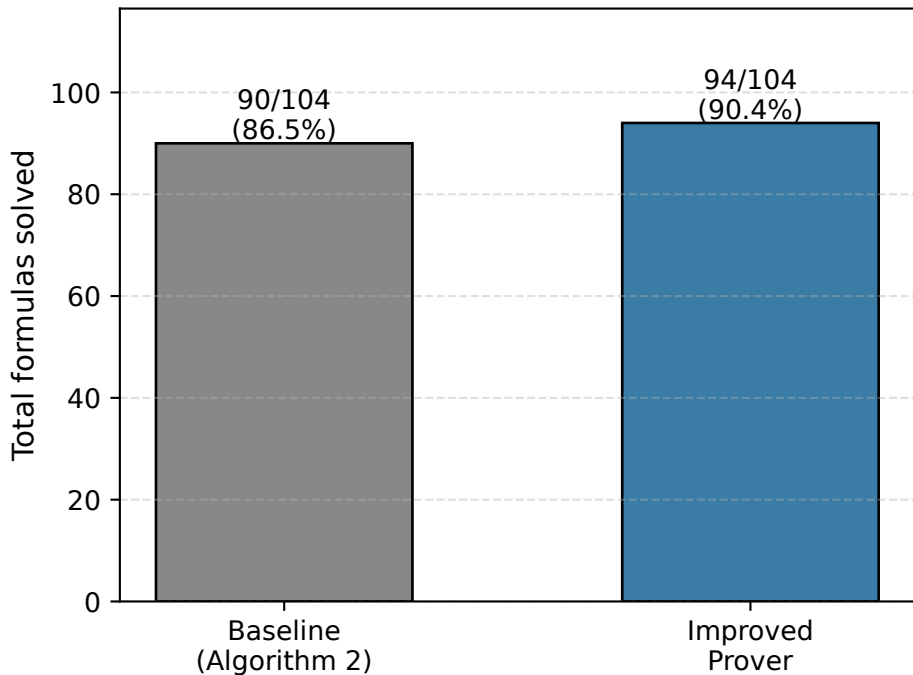
Overall Performance (across 104 formulas)
