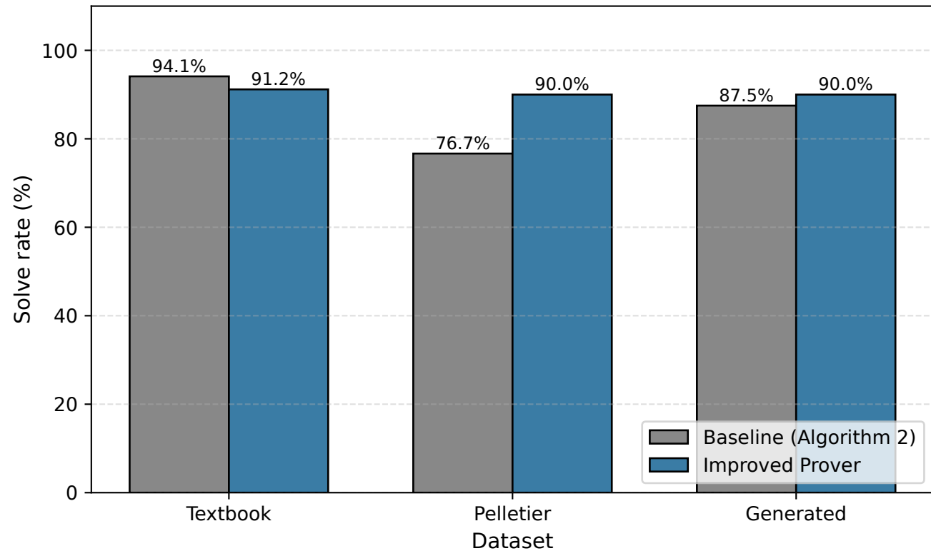
Solve Rate per Dataset
