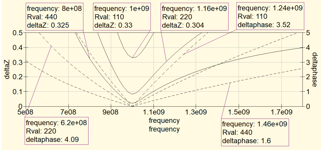
Figure 1: Difference in amplitude in \Omega (solid) and phase in degree (dashed) between a parallel and series circuit as a function of frequency in Hz for different resistances Rval
