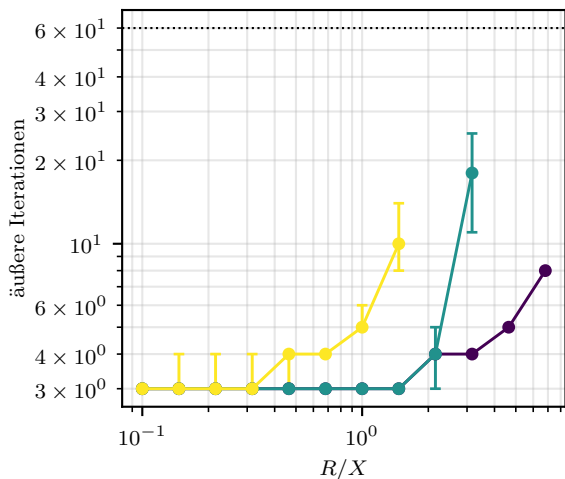
(c) const_x: Iterationen
