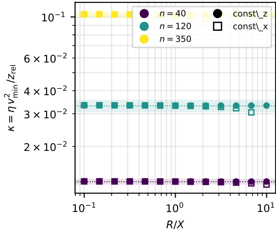
(a) Kollaps beider Modi, \pm Streuband
