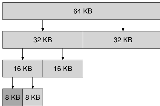
Figure 17.8: Example Buddy-managed Heap
