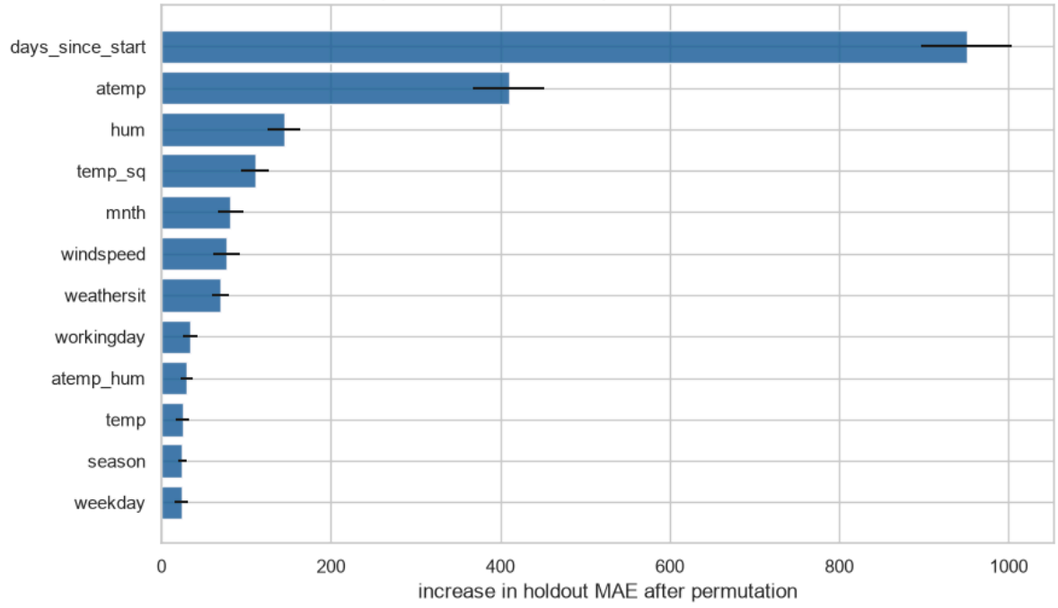
Figure 12 - Permutation importance: Gradient Boosting
