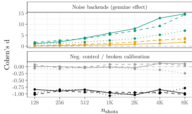
(a) Effect size vs. shot count
