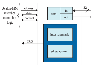
Figure 104. PIO Core with Input Ports, Output Ports, and IRQ Support
