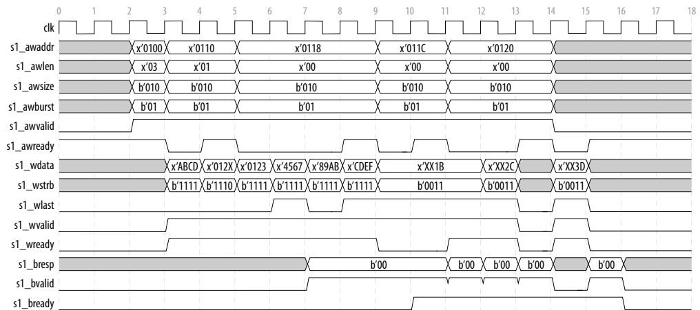
Figure 96. AXI Write with Back Pressure (BREADY Back Pressure)
