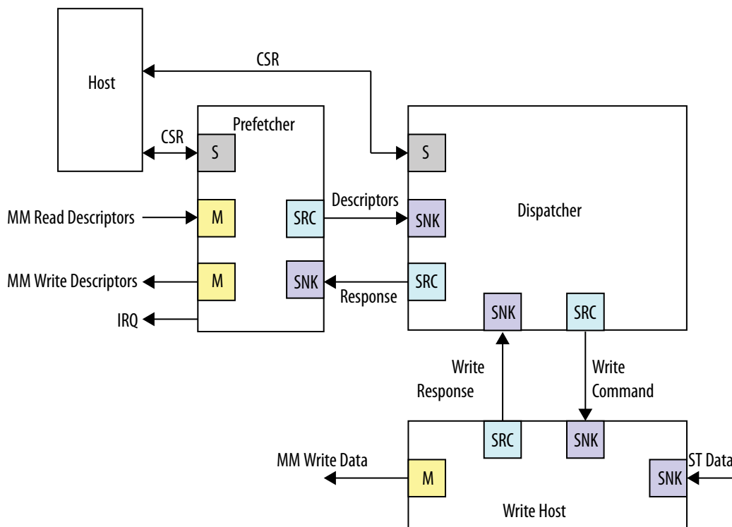
Figure 114. Streaming to Memory-Mapped Configuration with Prefetcher Enabled
