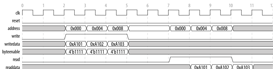
Figure 91. Avalon Memory-Mapped Write and Read with Clock Enable
