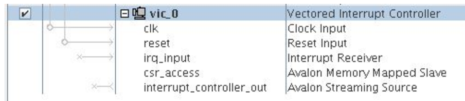
Figure 142. VIC Interfaces
