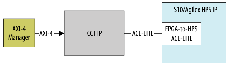
Figure 185. Cache Coherency Translator (CCT) Use Case
