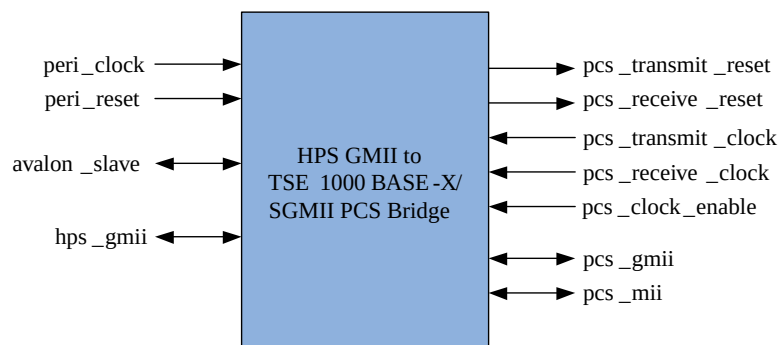
Figure 180. HPS GMII to TSE 1000BASE-X/SGMII PCS Bridge Intel FPGA IP Top Level Interfaces
