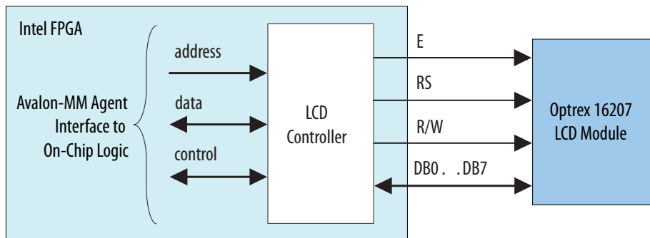
Figure 102. LCD Controller Block Diagram
