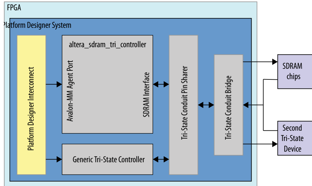
Figure 127. Shared-Bus System
