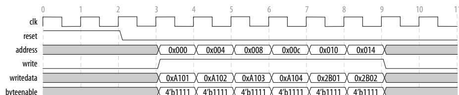
Figure 89. Avalon Memory-Mapped Write
