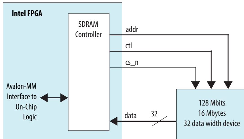
Figure 121. Single 128-Mbit SDRAM Chip with 32-Bit Data
