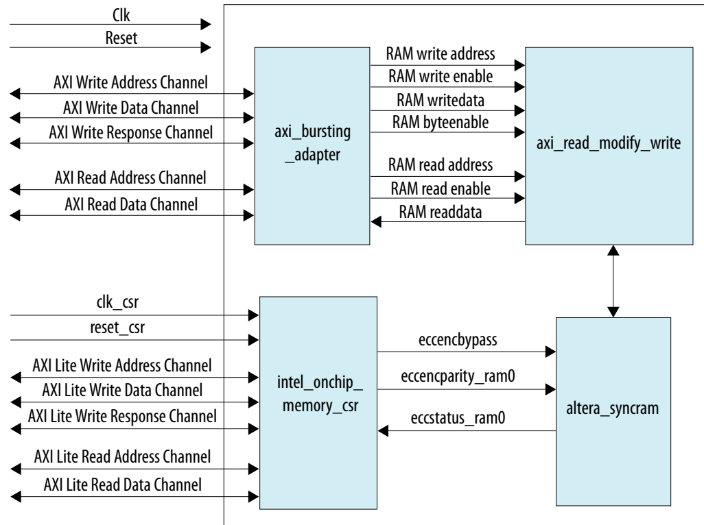
Figure 85. Block Diagram With AXI Interface When ECC Feature is Enabled
