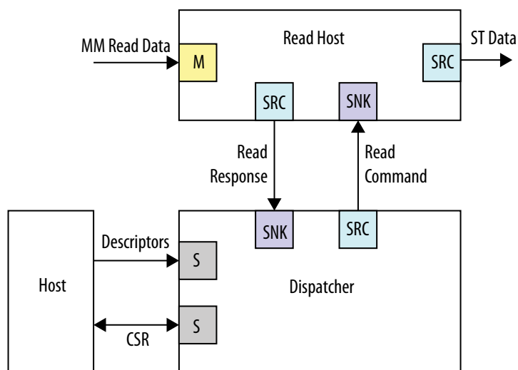
Figure 109. mSGDMA Module Configuration with Support for Memory-Mapped Streaming Reads to the Avalon-ST data bus
