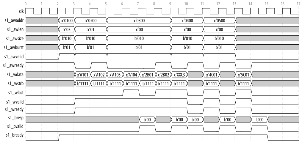
Figure 94. AXI Write with INCR Burst
