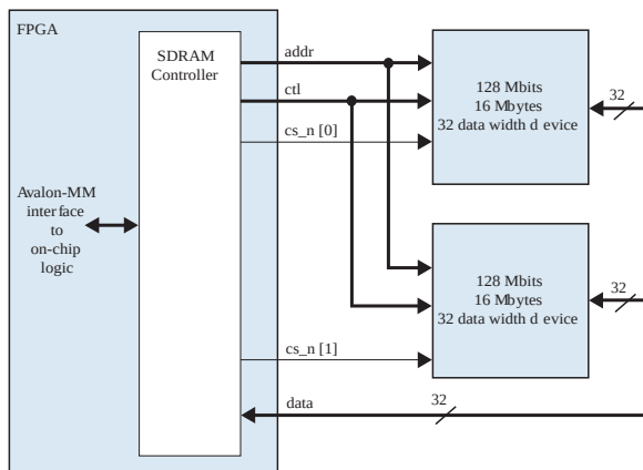
Figure 123. Two 128-Mbit SDRAM Chips Each with 32-Bit Data
