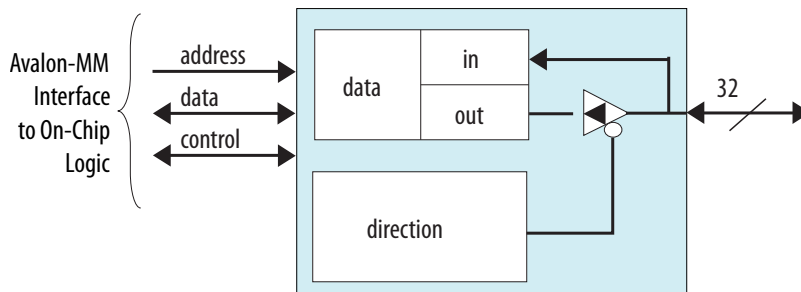
Figure 105. PIO Cores with Bidirectional Ports
