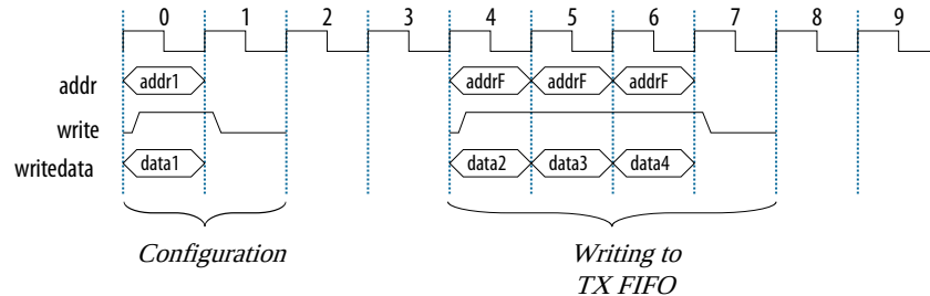
Figure 37. Writing to UART over Avalon-MM
