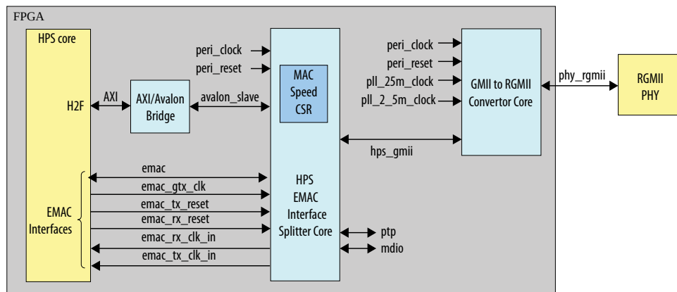
Figure 163. System Level Block Diagram
