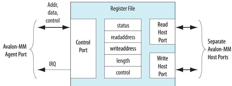
Figure 107. DMA Controller Block Diagram
