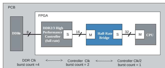
Figure 160. Platform Designer Memory System Using a DDR Memory Half-Rate Bridge
