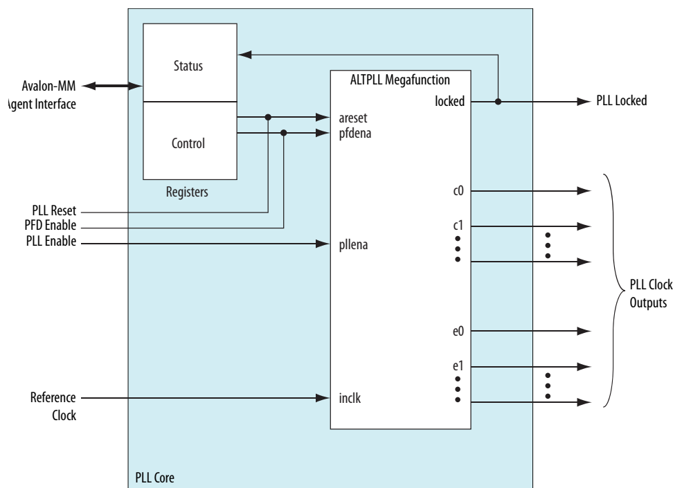
Figure 106. PLL Core Block Diagram
