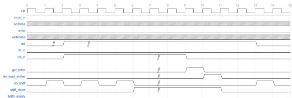
Figure 196. Flow Control in Lightweight UART Transmitter
