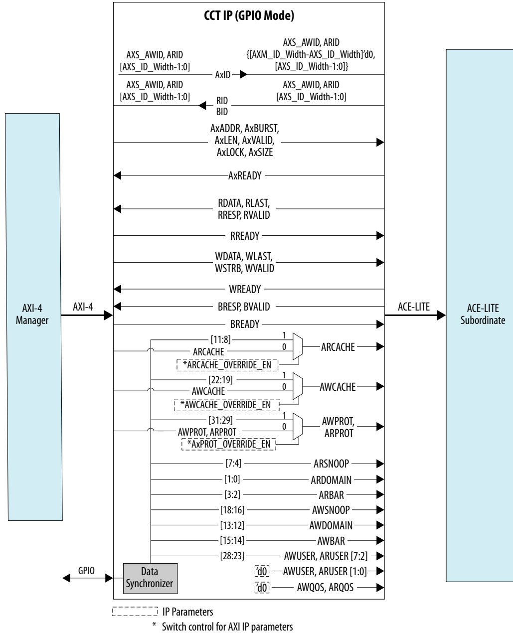
Figure 190. Block Diagram for GPIO Mode
