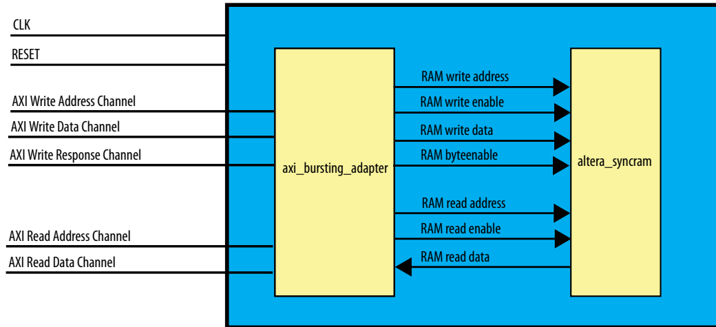
Figure 84. Block Diagram with AXI Interface
