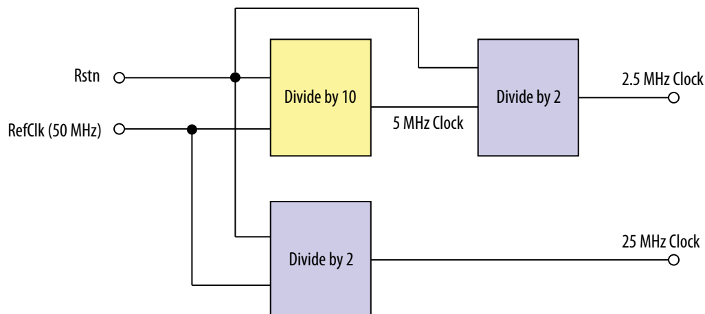
Figure 172. Clocking Scheme
