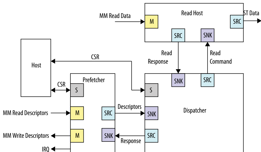
Figure 113. Memory-Mapped to Streaming Configuration with Prefetcher Enabled
