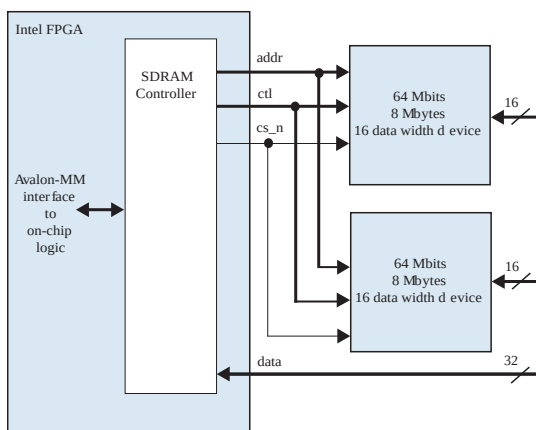
Figure 122. Two 64-MBit SDRAM Chips Each with 16-Bit Data
