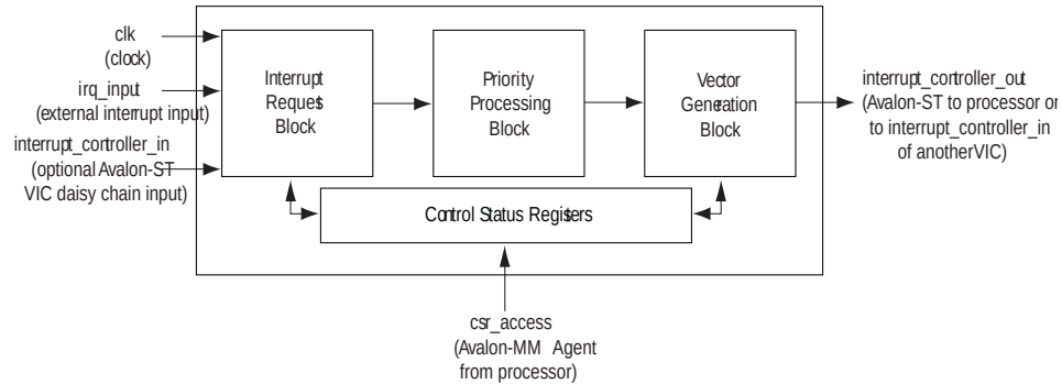
Figure 136. VIC Block Diagram
