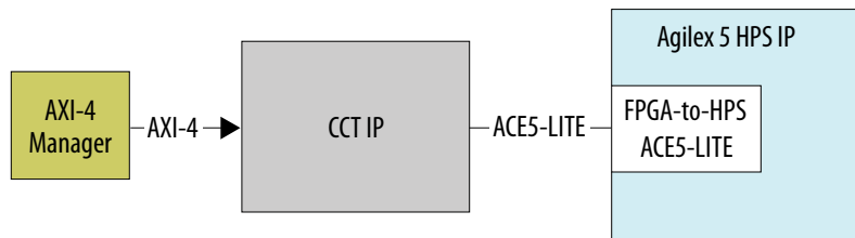
Figure 192. Cache Coherency Translator (CCT) Use Case
