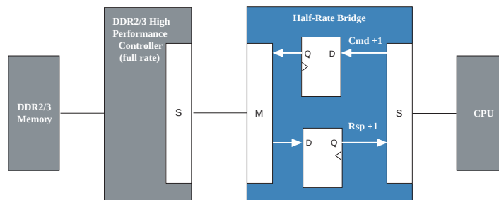
Figure 161. Avalon-MM DDR Memory Half-Rate Bridge Block Diagram
