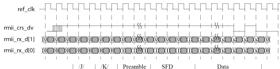
Figure 175. RMII Receive Transfer
