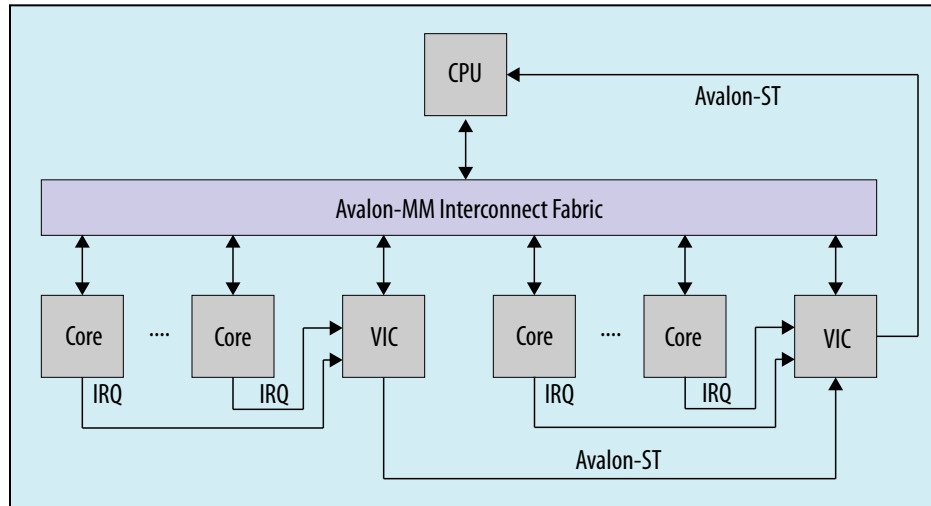
Figure 135. Sample System Layout
