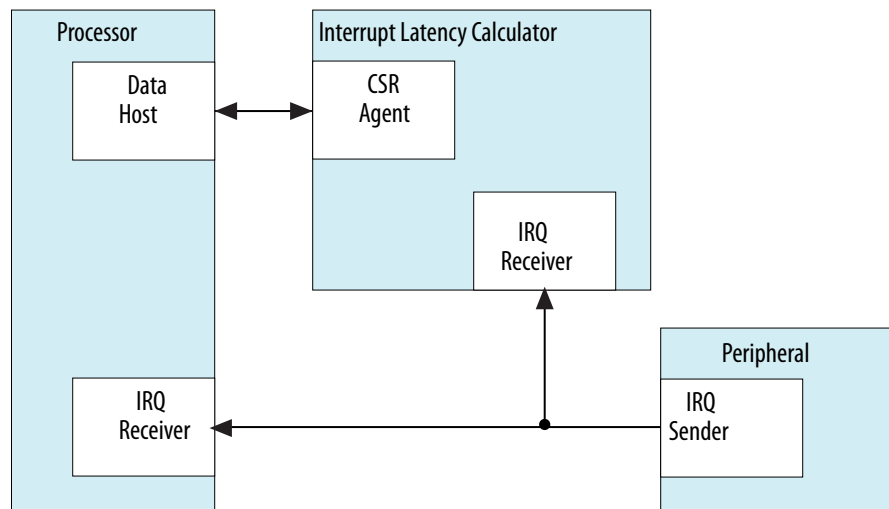
Figure 133. Usage model of Interrupt Latency Calculator
