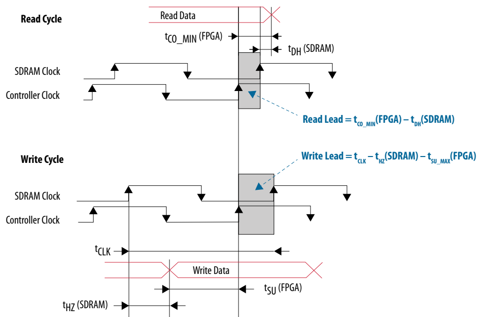
Figure 125. Calculating the Maximum SDRAM Clock Lead
