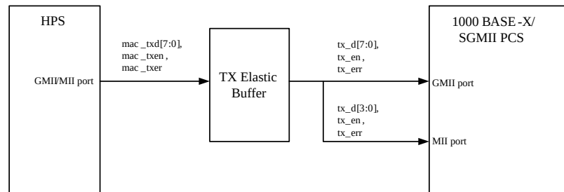
Figure 177. Transmit Data Path
