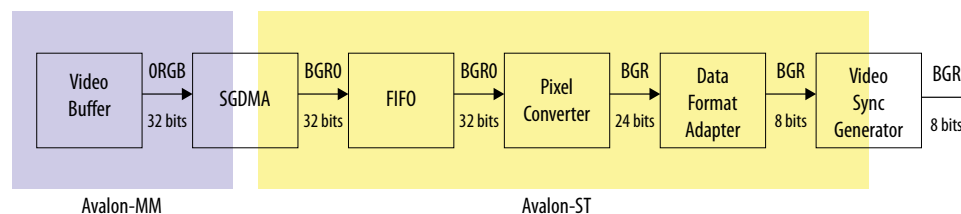
Figure 128. Typical Placement in a System
