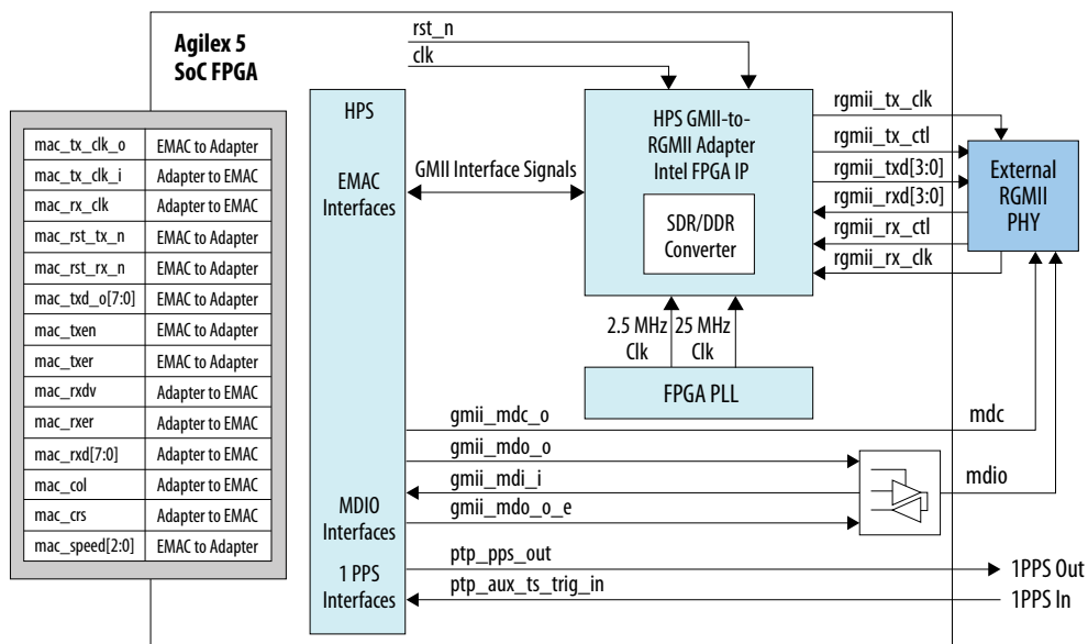
Figure 168. System Level Block Diagram
