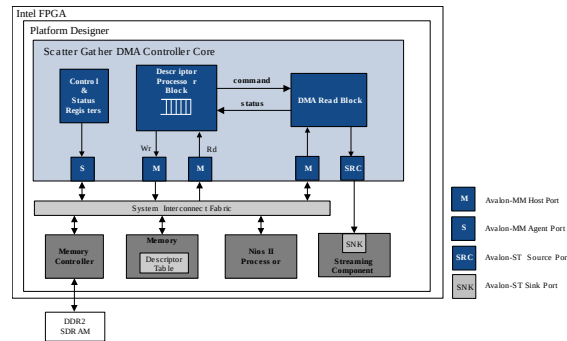
Figure 118. Example of Memory-to-Stream Configuration
