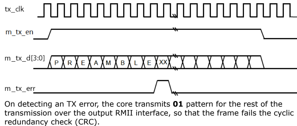
Figure 174. TX Frame with Error Signal
