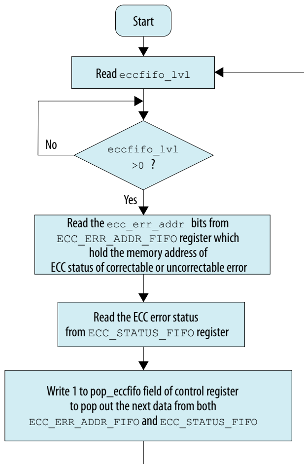
Figure 99. Programming Flow to Read ECC Error Status FIFO
