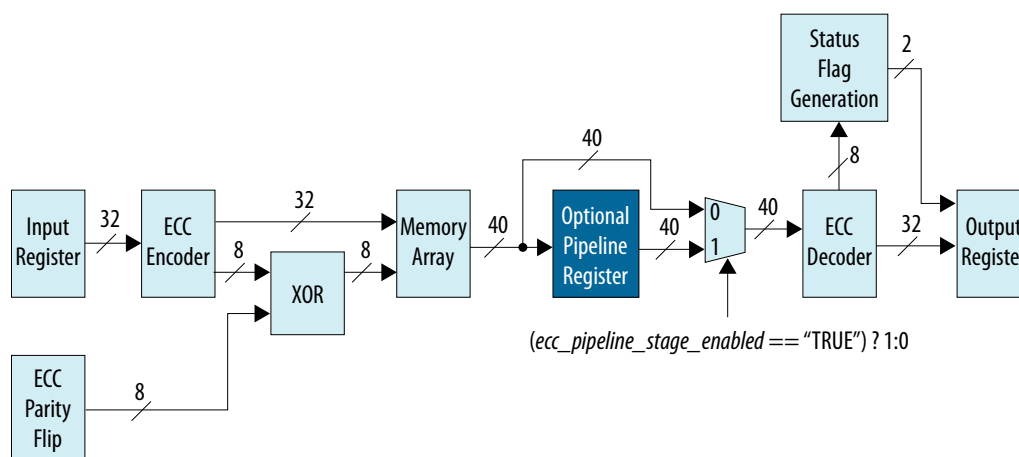
Figure 87. ECC Block Diagram for M20K Memory
