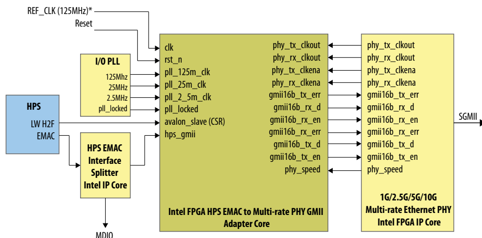
Figure 181. Block Diagram
