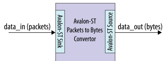
Figure 155. Avalon-ST Packets to Bytes Converter Core
