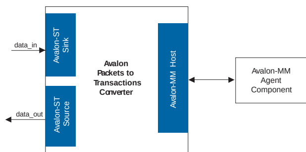
Figure 150. Avalon Packets to Transactions Converter Core
