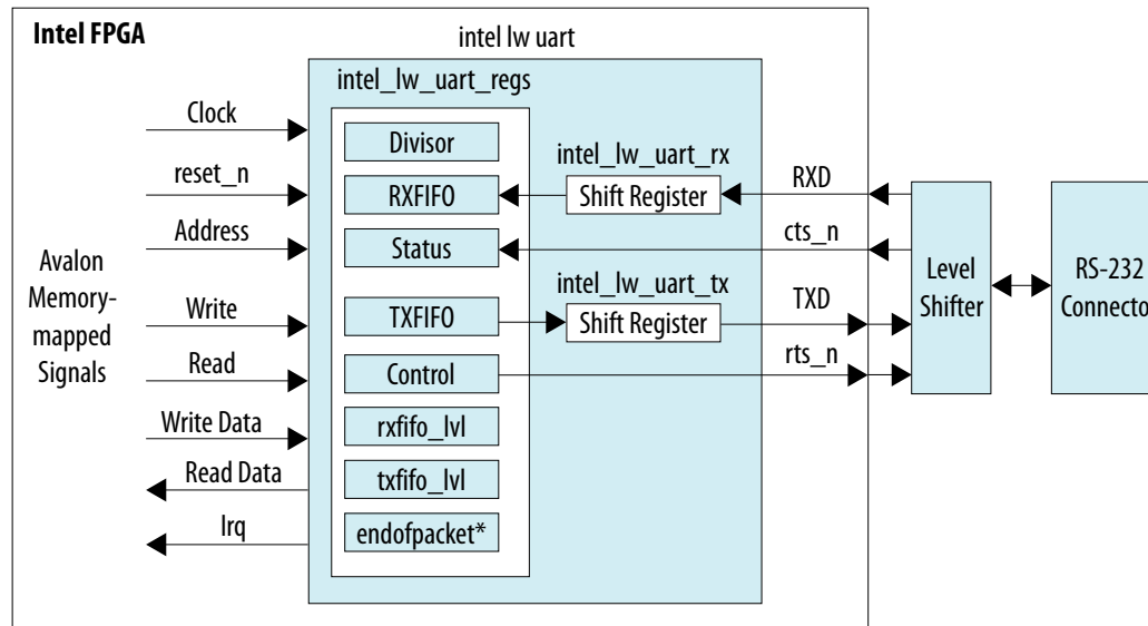
Figure 195. Block Diagram of Lightweight UART Core in a Typical System
