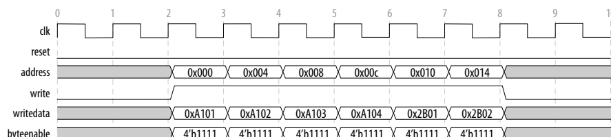
Figure 89. Avalon Memory-Mapped Write
