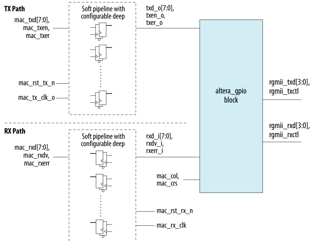
Figure 169. Transmit and Receive Data Path
