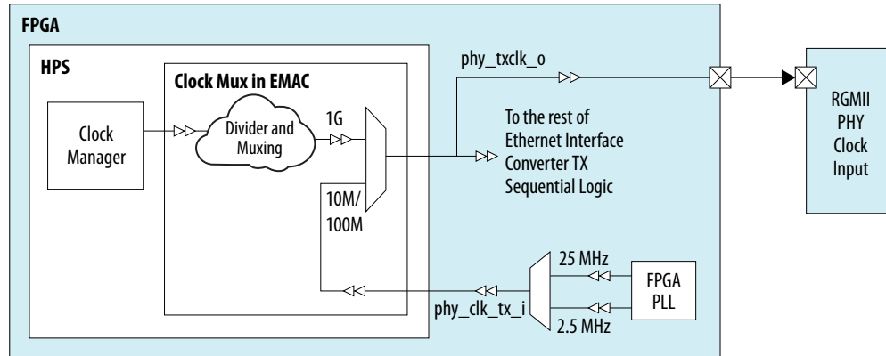
Figure 170. Transmit Clocking Scheme
