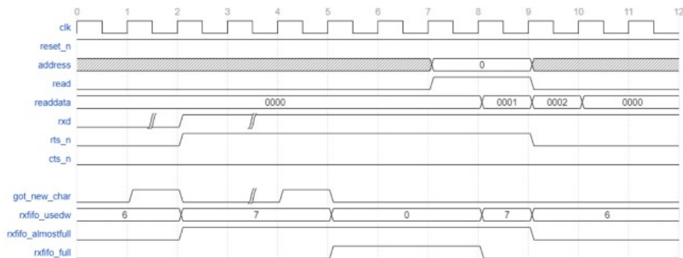
Figure 197. Flow Control in Lightweight UART Receiver
