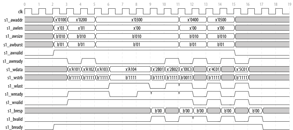
Figure 95. AXI Write with Back Pressure (WVALID back pressure)
