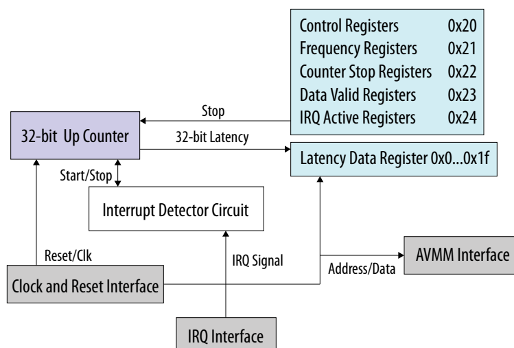
Figure 134. Interrupt Latency Calculator Architecture
