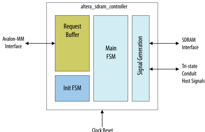
Figure 126. Tri-State SDRAM Block Diagram
