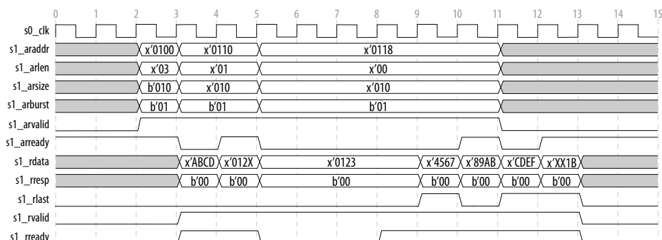
Figure 97. AXI Read with Back Pressure (RREADY)
