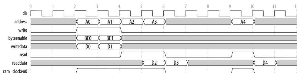
Figure 83. Clock Enable Timing Diagram for Avalon Memory-Mapped based Interface
