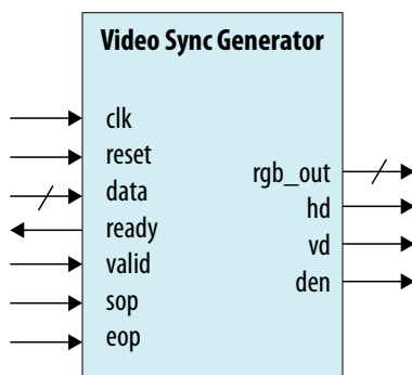
Figure 129. Video Sync Generator Block Diagram
