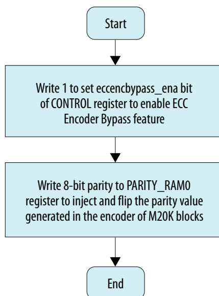
Figure 100. Programming Flow to Enable Encoder Bypass Feature
