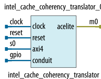
Figure 187. GPIO Mode Block Diagram (CONTROL_INTERFACE = 1 (GPIO))
