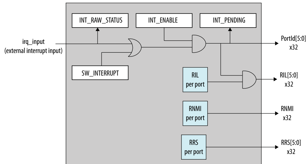
Figure 137. Interrupt Request Block
