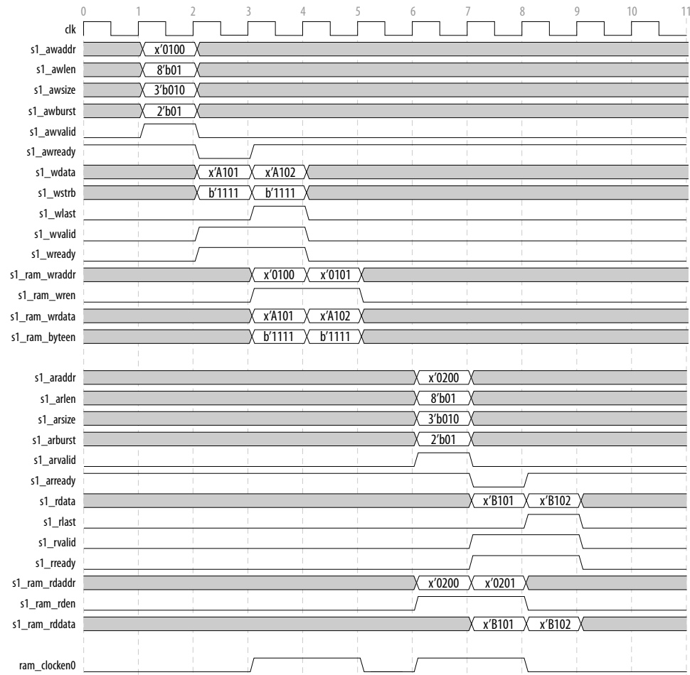
Figure 86. Clock Enabled Timing Diagram for AXI-4 Based Interface
