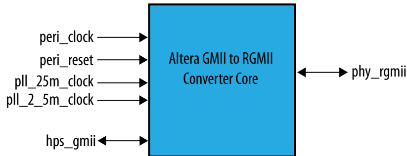
Figure 162. Intel FPGA GMII to RGMII Converter Core Top Level Interfaces
