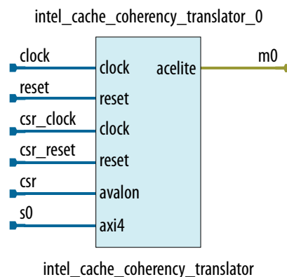
Figure 188. CSR Mode Block Diagram (CONTROL_INTERFACE = 2 (CSR))
