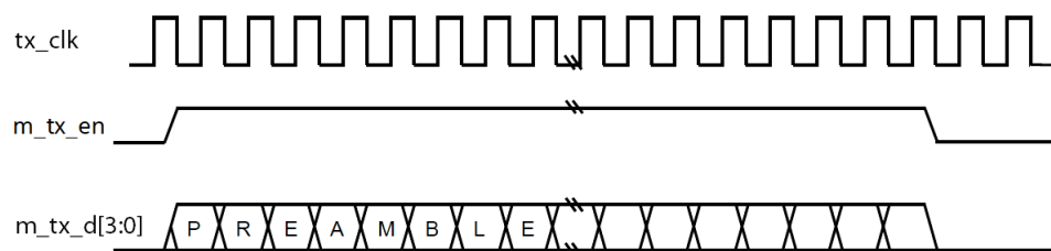
Figure 173. MII TX Frame
