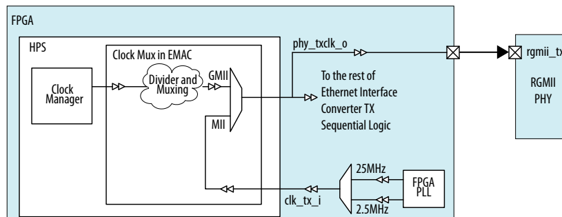
Figure 165. Transmit Clocking Scheme
