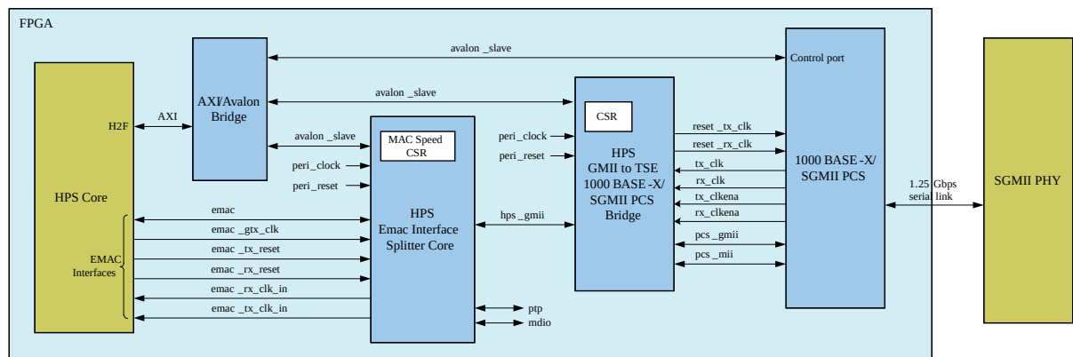
Figure 176. HPS GMII to TSE 1000BASE-X/SGMII PCS Bridge Intel FPGA IP Core Block Diagram
