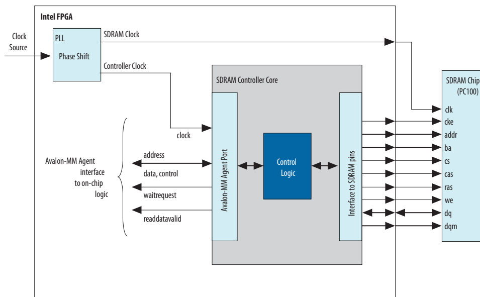
Figure 120. SDRAM Controller with Avalon Interface Block Diagram
