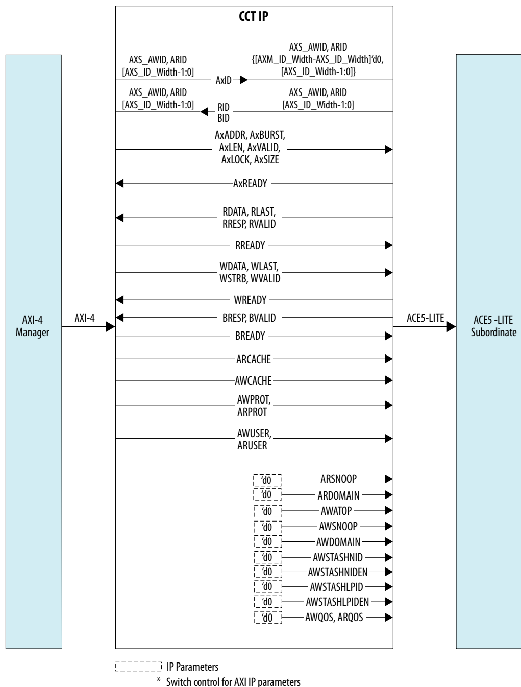
Figure 194. Detailed Block Diagram
