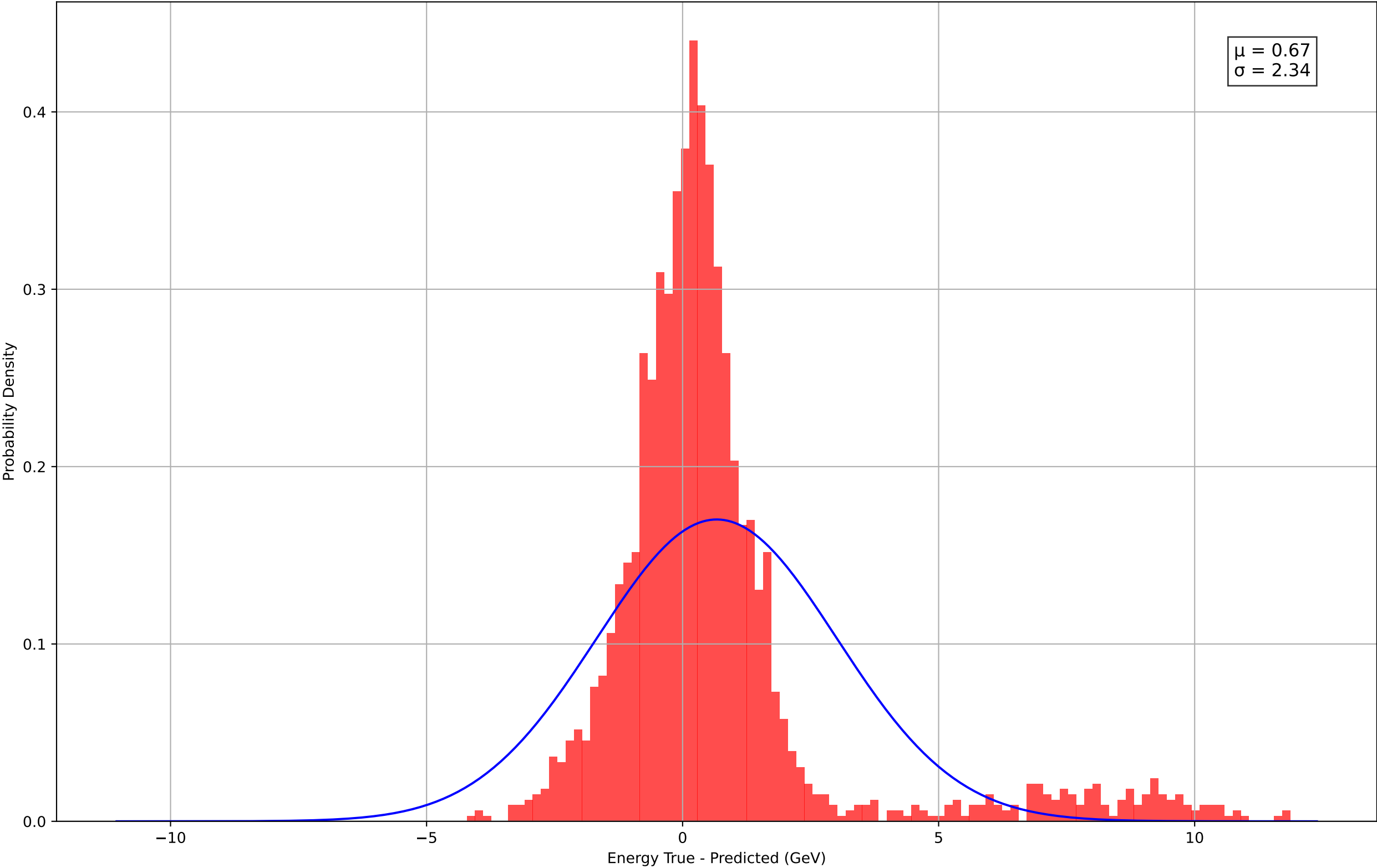
Energy Residuals (13.0-14.0 GeV)
